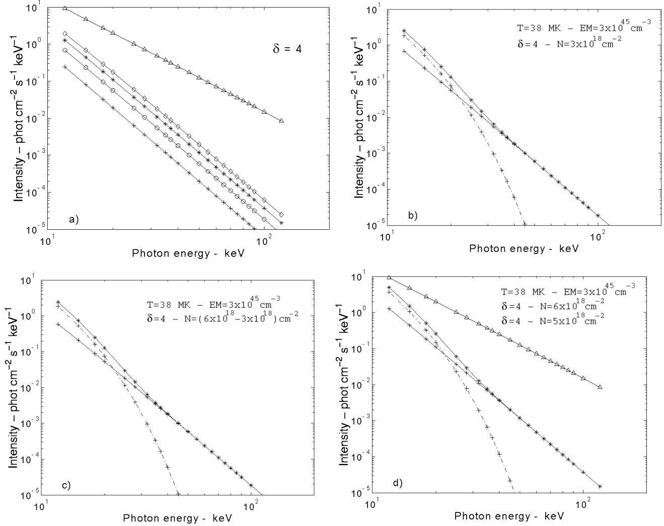
Fig. 1. (a) Total non thermal HXR yield (from N = 0 ) at different column densities, N ( \text{cm}^{-2} ), from bottom to top: N = 1.0 \times 10^{18} \text{ cm}^{-2} (crosses), N = 3.0 \times 10^{18} \text{ cm}^{-2} (circles), N = 6.0 \times 10^{18} \text{ cm}^{-2} (asterisks), N = 1.0 \times 10^{19} \text{ cm}^{-2} (diamonds), N = 5.0 \times 10^{22} \text{ cm}^{-2} (triangles). Note the hardening of the highest spectrum, that corresponds to emission from the chromospheric footpoint. (b) Total HXR yield from injection up to N = 3.0 \times 10^{18} \text{ cm}^{-2} (continuous line and crosses), the thermal contribution from the 3.8 \times 10^7 \text{ K} plasma (dash-dotted line and crosses) for an emission measure of EM = 10^{45} \text{ cm}^{-3} , and the summation of both contributions (continuous line and asterisks). (c) Same as (b), for 3.0 \times 10^{18} \leq N \leq 6.0 \times 10^{18} \text{ cm}^{-2} (same convention as in Fig. 1b). (d) Total HXR yield of the looptop ( 0 \leq N \leq 6.0 \times 10^{18} \text{ cm}^{-2} ), including the hot plasma thermal contribution (same convention as in Fig. 1b). Added the chromospheric footpoint contribution, N = 5.0 \times 10^{22} \text{ cm}^{-2} (continuous line and diamonds).
