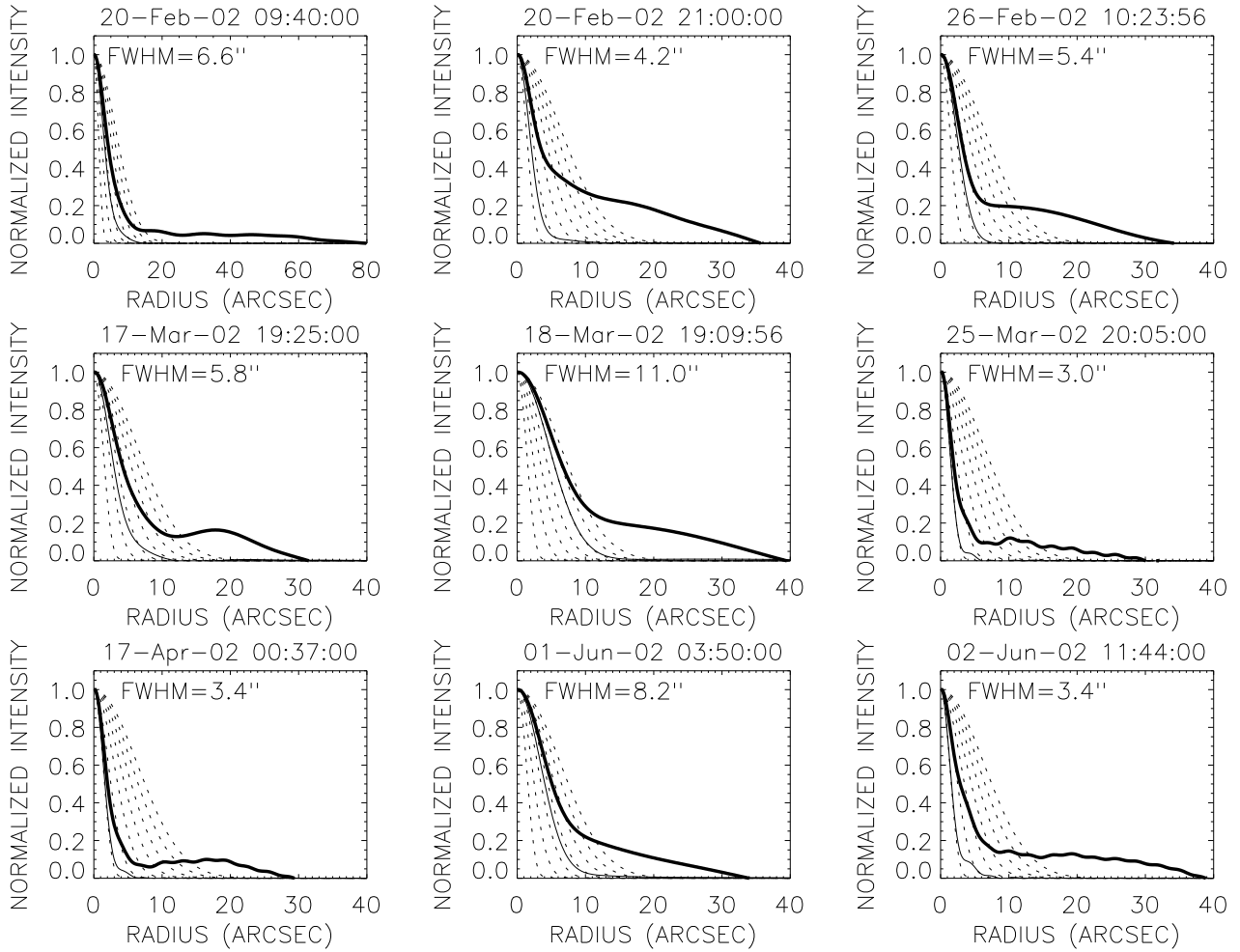
Fig. 3. Spatial profiles inferred for 9 flares. The relative amplitude profiles (Figure 2) were Fourier transformed to obtain the spatial profiles l(r) shown as the light solid curves. Dashed curves show representative Gaussians (FWHM=3, 5, 7, ..., 15'') transformed from the dashed Gaussians of Figure 2. The heavy curves show the integrated flux outside the radius. The difference between it and l(r) indicates extended flux beyond the cores.
