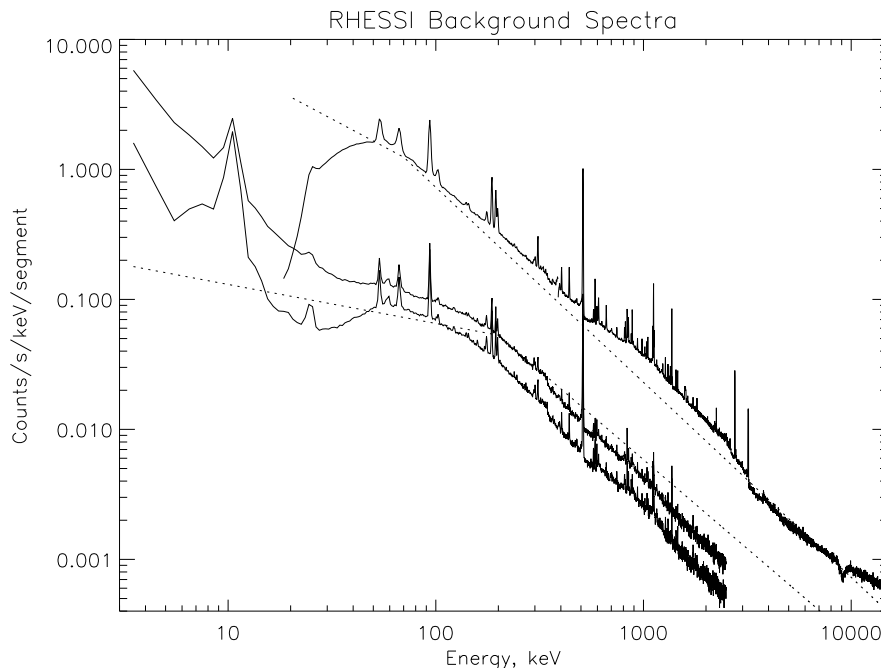
Figure 9. Typical RHESSI background spectra, accumulated over 2.5 hr. The three solid traces, top to bottom, are the backgrounds in the rear segments, the front segments, and the front segments using front/rear anticoincidence (“phoswich mode”). The dotted lines are pre-flight predictions of the background that included continuum from the cosmic diffuse background and from cosmic rays interacting in the Earth’s atmosphere and in the spacecraft.
