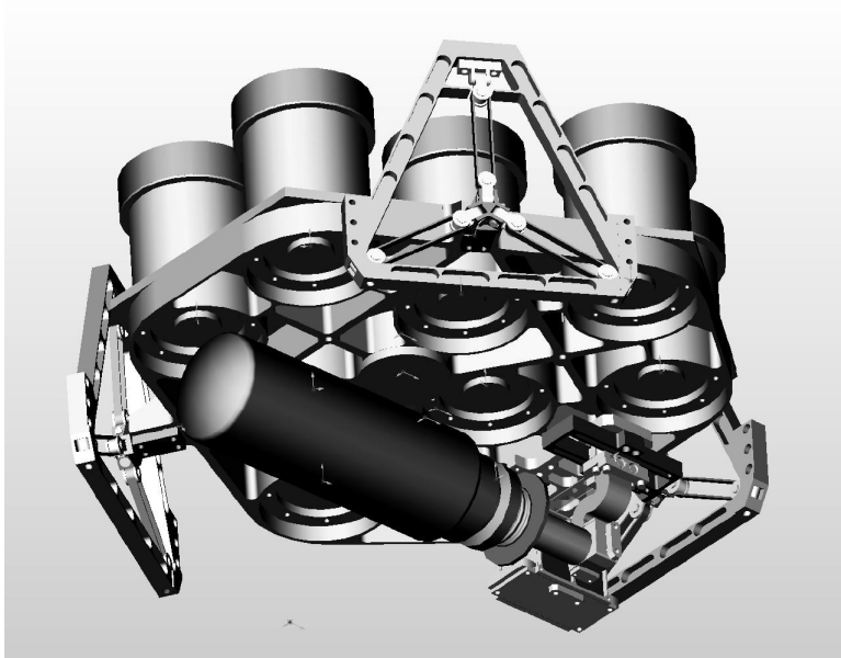
Figure 5. The interior of the RHESSI spectrometer, showing the detectors mounted on the coldplate, the Sunpower cryocooler below it, and the fiberglass-strap “cartwheels” that suspend this assembly in the interior of the cryostat.
