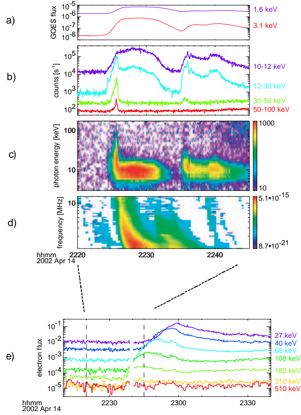
Figure 2. Time profile of X-ray fluxes from GOES ((a)top panel) and RHESSI ((b)next panel; counts are multiplied by factors of 8, 50, and 500, for the 30-50 keV, 12-30 keV, and 10-12 keV channels, respectively). The next two panels show spectrograms of (c)the RHESSI counts in 20 logarithmic energy channels, and of (d)1-14 MHz radio emission detected by the Wind spacecraft (Bougeret et al, 1995). The solar flare with hard X-ray peak at \sim 2226 UT is accompanied by a type III solar radio burst, produced by energetic electrons escaping the Sun. The (e)bottom panel (longer time interval) shows the energetic electron arriving at Wind at 1 AU (Lin et al, 1995), with the faster electrons arriving first, consistent with an impulsive injection of the electrons from the Sun at the time of the X-ray peak
