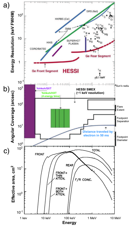
Figure 4. a) RHESSI's FWHM energy resolution (lower curves), compared with previous instruments (upper lines). The dots are the expected FWHM widths of the predicted gamma-ray lines, and the vertical line the range of widths (temperature and density dependent) for the positron annihilation line. The short diagonal line shows the resolution needed to resolve the steep "superhot thermal" emission. b) RHESSI's angular resolution versus energy, compared to Yohkoh SXT (left) and HXT (center). RHESSI has \sim 1 -10 keV energy resolution over this energy range and can image up to 17 MeV, while HXT has four broad energy channels from 15 to 100 keV. (c) RHESSI's effective (photopeak) area as a function of energy for solar X-rays/gamma-rays. The three curves to the left show the effect on the front segment response (summed over all nine detectors) of no attenuators, thin attenuator, or both thick and thin attenuator inserted over the detectors. The curves to the right show the effective area for the rear segment, and for photons that leave energy in both the front and rear segment of the detectors (F/R coincidence).
