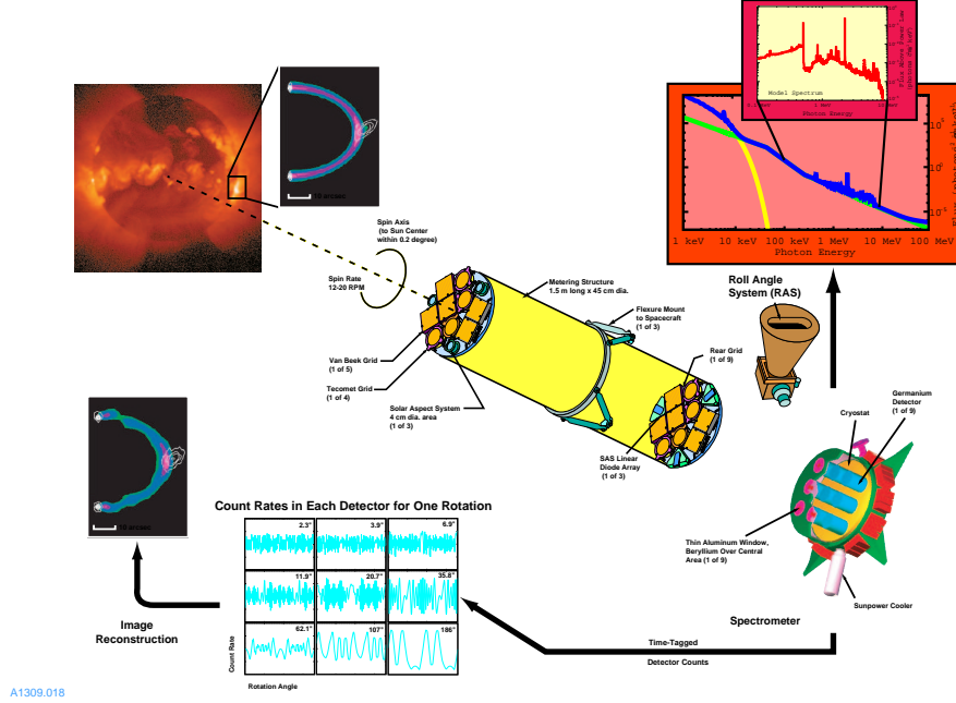
Figure 5. Schematic of the RHESSI instrument illustrating the imaging spectroscopy. X-rays and gamma-rays from the Sun (upper left) pass through the slits of the front and rear grids of each of the nine grid pairs to reach the germanium detector. As the spacecraft rotates the detector count rates are temporally modulated (lower left). These modulations can be analyzed to reconstruct the image. The germanium detectors are cryogenically cooled to provide high spectral resolution capable of resolving narrow gamma-ray lines and steep solar continuum spectra (upper right). The attenuators are inserted automatically when the count rate approaches saturation. The SAS and RAS provide solar pointing and roll aspect information.
