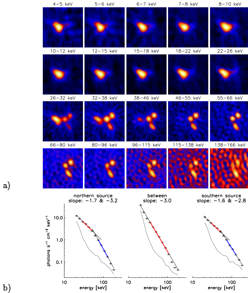
Figure 3. a) Imaging of the July 23, 2002, X4.8 solar flare in 20 energy bands, from 1 keV wide bins at 4 keV, to 28 keV wide (for enough counts to image) at 138 keV, illustrating the changes in sources as a function of energy. The images are 64 arcseconds on a side. b) The energy spectra of the three dominant sources at energies above \sim 40 keV, showing that the spectra are similar for the north and south sources but quite different for the source in between.
