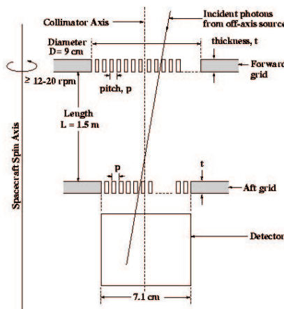
Figure 6. Schematic showing the parameters that define the imaging capability
