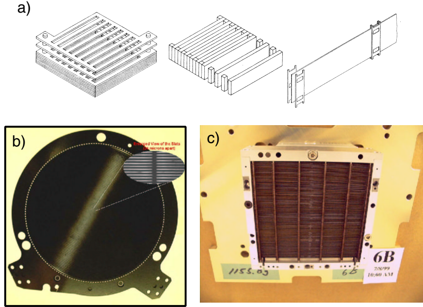
Figure 7. a) Schematic of the two grid fabrication processes: left, stacking etched foils and epoxying them to obtain the required thickness; middle and right, packing vertical blades with spacers in between. b) Photograph of a grid #1 showing the slits and bridges in the insert. c) Photograph of flight grid #6.
