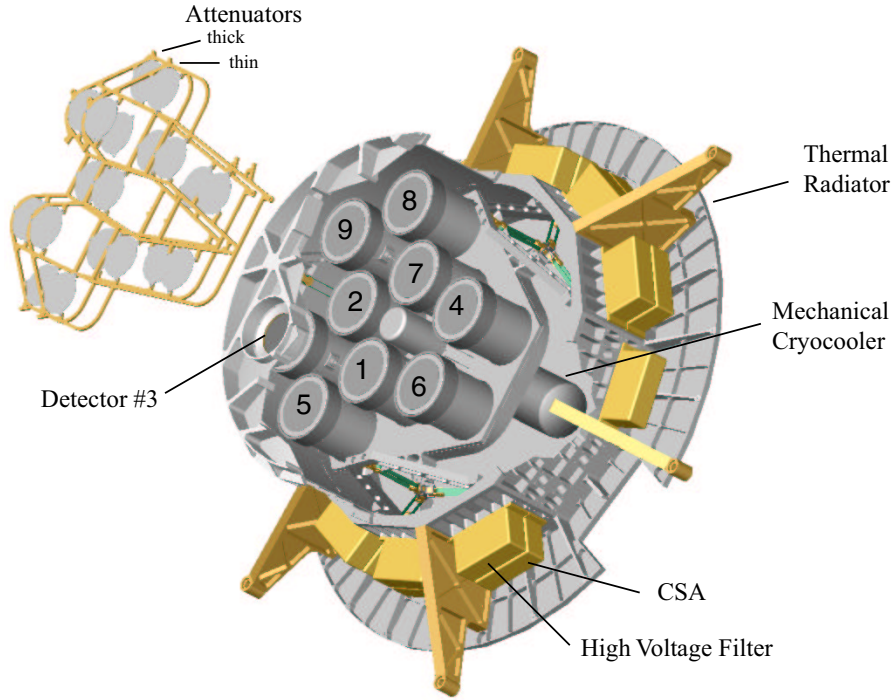
Figure 8. A cutaway of the Spectrometer, showing the location of the germanium detectors under each grid (by number). The Sunpower Stirling-cycle mechanical cooler is below the cold plate holding the detectors. The thermal radiator faces anti-sunward to reject the heat of the cryocooler. The attenuators are automatically moved in when the counting rate exceeds thresholds (commandable from the ground).
