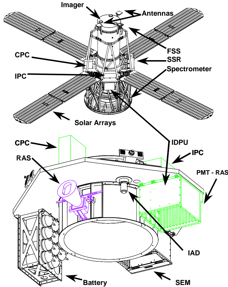
Figure 10. Schematic showing the location of instrument and spacecraft components on the RHESSI spacecraft. The acronyms in the top view are: Fine Sun Sensor (FSS), Solid State Recorder (SSR), Cryocooler Power Converter (CPC), Instrument Power Converter (IPC), Instrument Data Processing Unit (IDPU); in the bottom view, Roll Angle System (RAS), Photomultiplier Roll Angle System (PMT RAS), Inertial Adjustment Device (IAD), Spacecraft Electronics Module (SEM).
