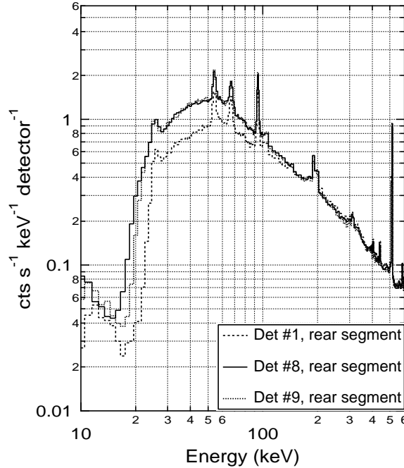
Figure 9. Measured background spectra for RHESSI detectors 1, 8 and 9.
