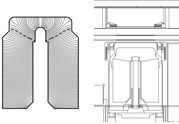
Figure 3. Cross section of a RHESSI detector. Left: A detector profile with field lines, the dashed field line indicating the separation between the front and back segments. Right: A detector in the cryostat, showing Ta/Sn/Fe/Al shielding around the side of the front segment and above the shoulder of the rear segment.
