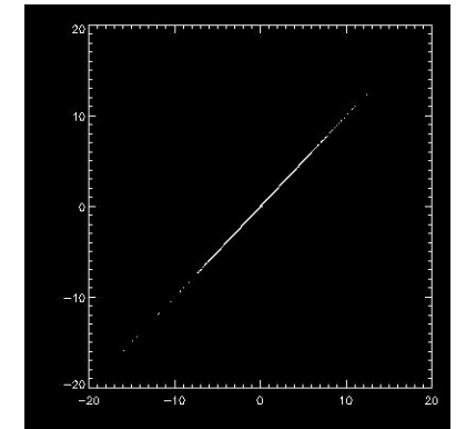
\partial B_x/\partial t vs \partial B_x/\partial t
