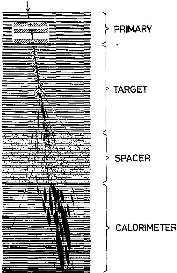
Figure 1. Schematic diagram of the JACEE emulsion chamber.
