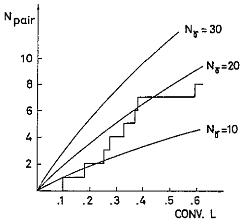
Figure 6. Integral distribution of conversion distances of the eight photons from the two decays (histogram). The curves show expected distributions for various initial numbers of photons, N_\gamma .
