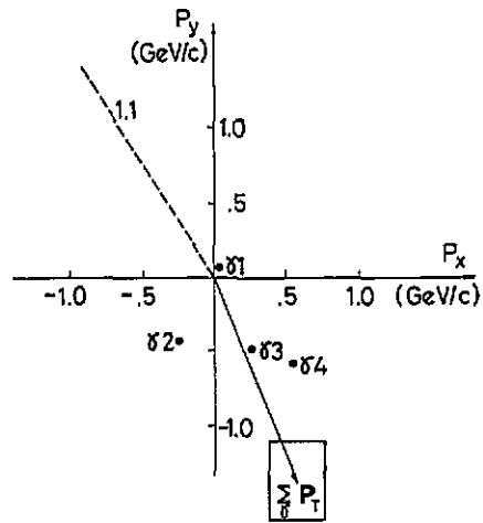
Figure 3. Transverse momentum balance of decay products of particle 1 in event 1. The rectangle shows error limits of p_T sum for electron pairs \gamma_1 , \gamma_2 , \gamma_3 , \gamma_4 . The broken line shows the direction of p_T of particle 1.1.
