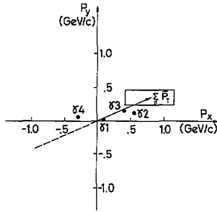
Figure 5. Transverse momentum balance of decay products of particle 1 in event 2. The notation is the same as in figure 3.
