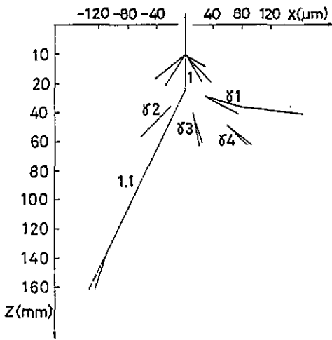
Figure 2. Projection of decay of particle 1 in event 1. \gamma_1 , \gamma_2 , \gamma_3 and \gamma_4 are electron pairs from photon conversions. The broken line shows the direction of track 1.1 before the kink.
