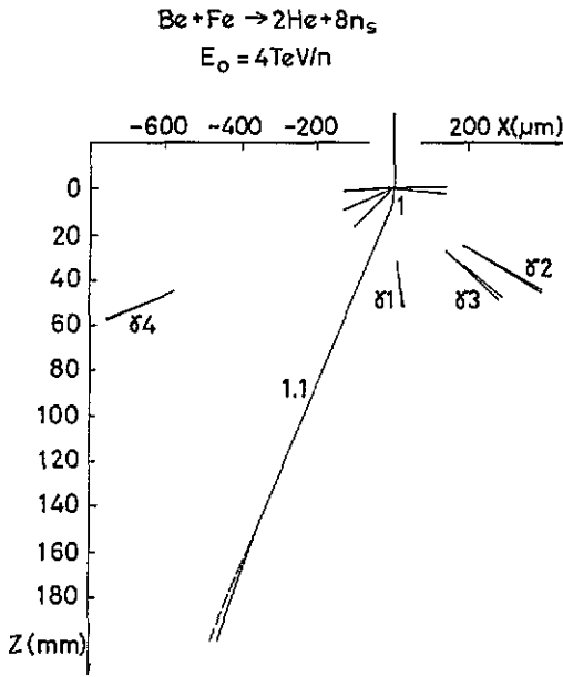
Figure 4. Decay of particle 1 in event 2. The notation is the same as in figure 2.
