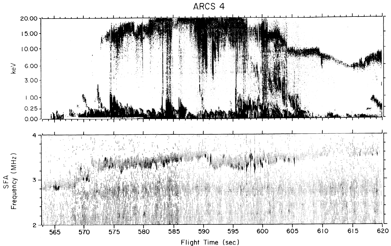
Figure 3. Energy spectrogram of energetic electron energy flux observed during the ARCS4 flight as the payload overflowed the bright auroral arc. In addition to the intense feature at high energy, a notable set of features is seen at the lowest energies, below \sim 250 eV.
