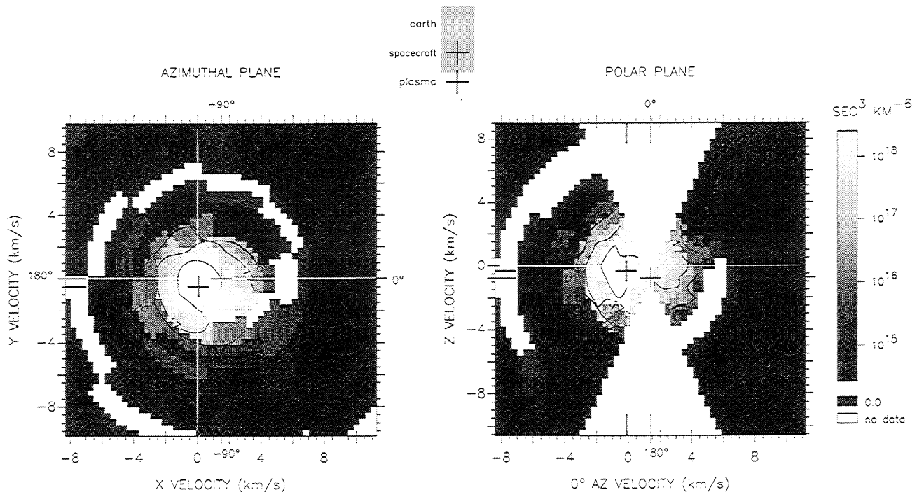
Figure 7. Three-dimensional representation of the O + velocity distribution for the period near 310 s. TAL of the ARCS-4 flight. The axes scale velocities relative to the Earth. Each data point is represented by a contoured value of the phase space density, arrayed in two panels representing cuts through the full velocity distribution in the plane perpendicular to the local magnetic field (left), and in a plane containing the local magnetic field (right). The bin structure contains 8 azimuths, 15 pitch angles, and 27 energies/speeds (radius). The azimuth of the cut in the right hand panel is indicated as 0°. The moments of the distribution are tabulated in the header documentation; velocities indicated include V_{ps} (plasma relative to spacecraft), V_{es} (Earth relative to spacecraft), and V_{pe} (plasma relative to Earth). A legend given at center indicates the crosshairs that mark the origins of the various coordinate systems: earth frame, spacecraft frame, and plasma frame.
