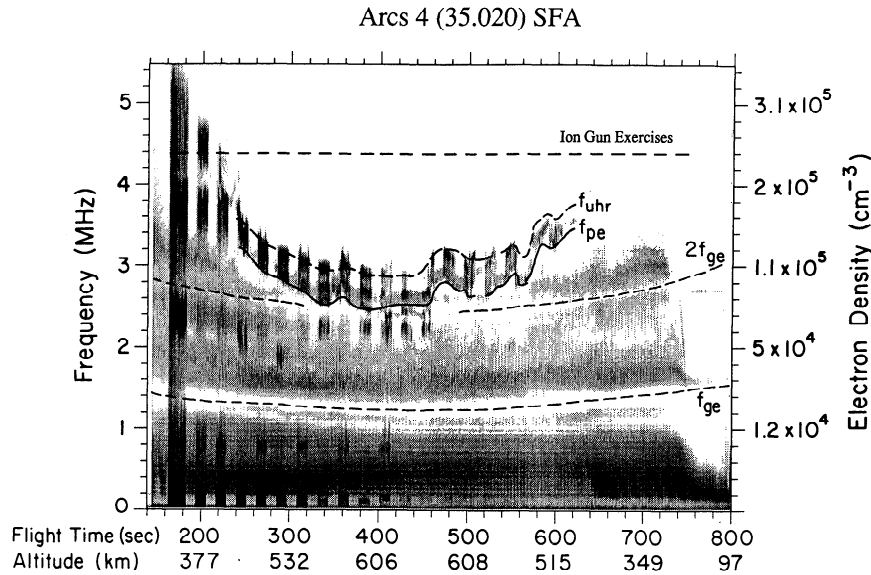
Figure 5. Spectrogram of high frequency electrostatic fluctuations observed at the ARCS4 main payload.
