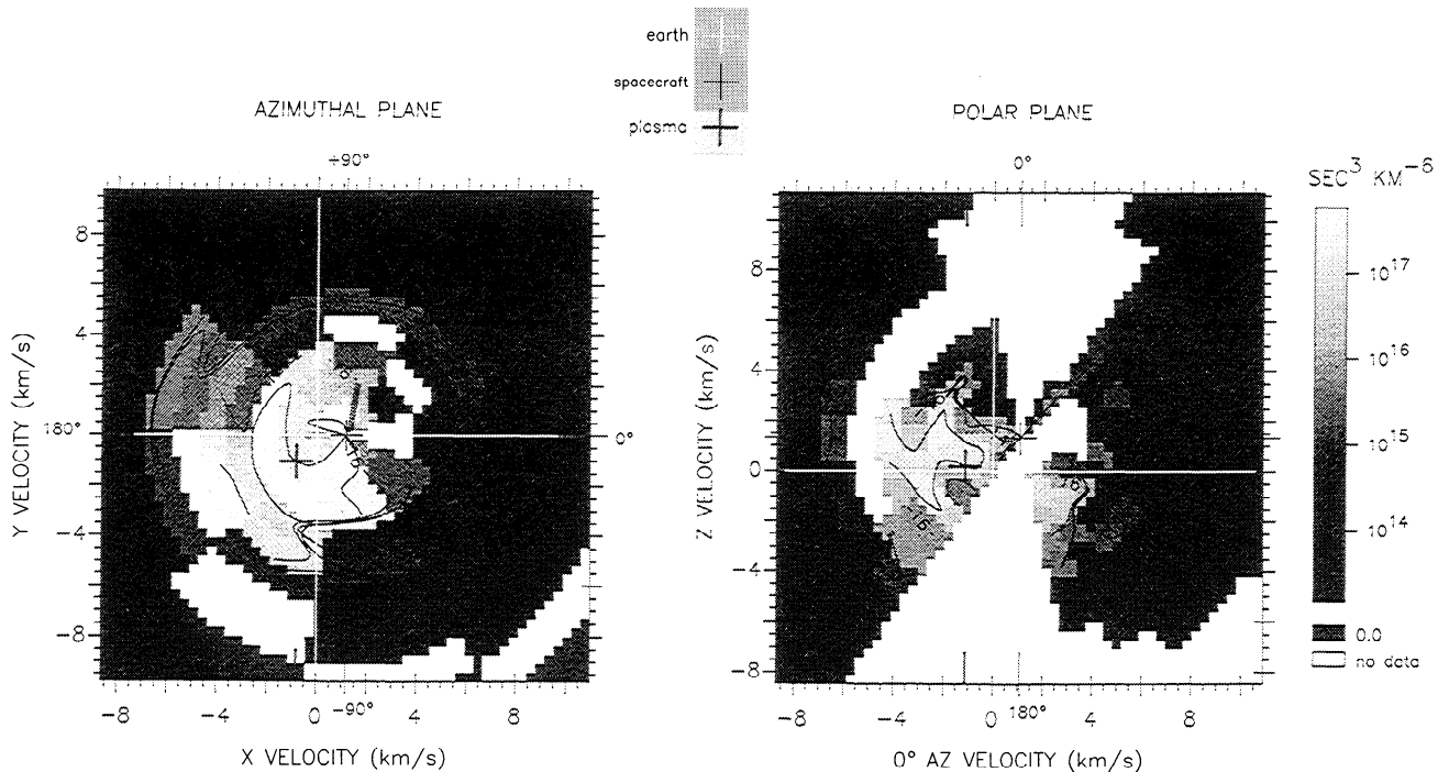
Figure 8. Similar to Figure 7., but giving the O + velocity distribution for the period near 585 s. TAL, as the payload entered the main auroral arc.
