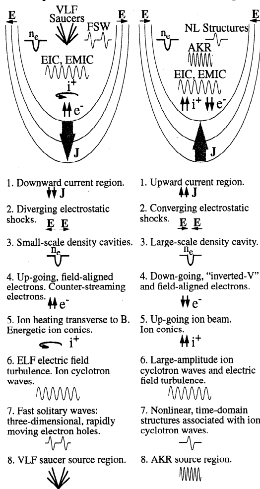
Figure 2. A schematic representation of the principle physical phenomena that characterize the upward and downward current regions in the aurora.
