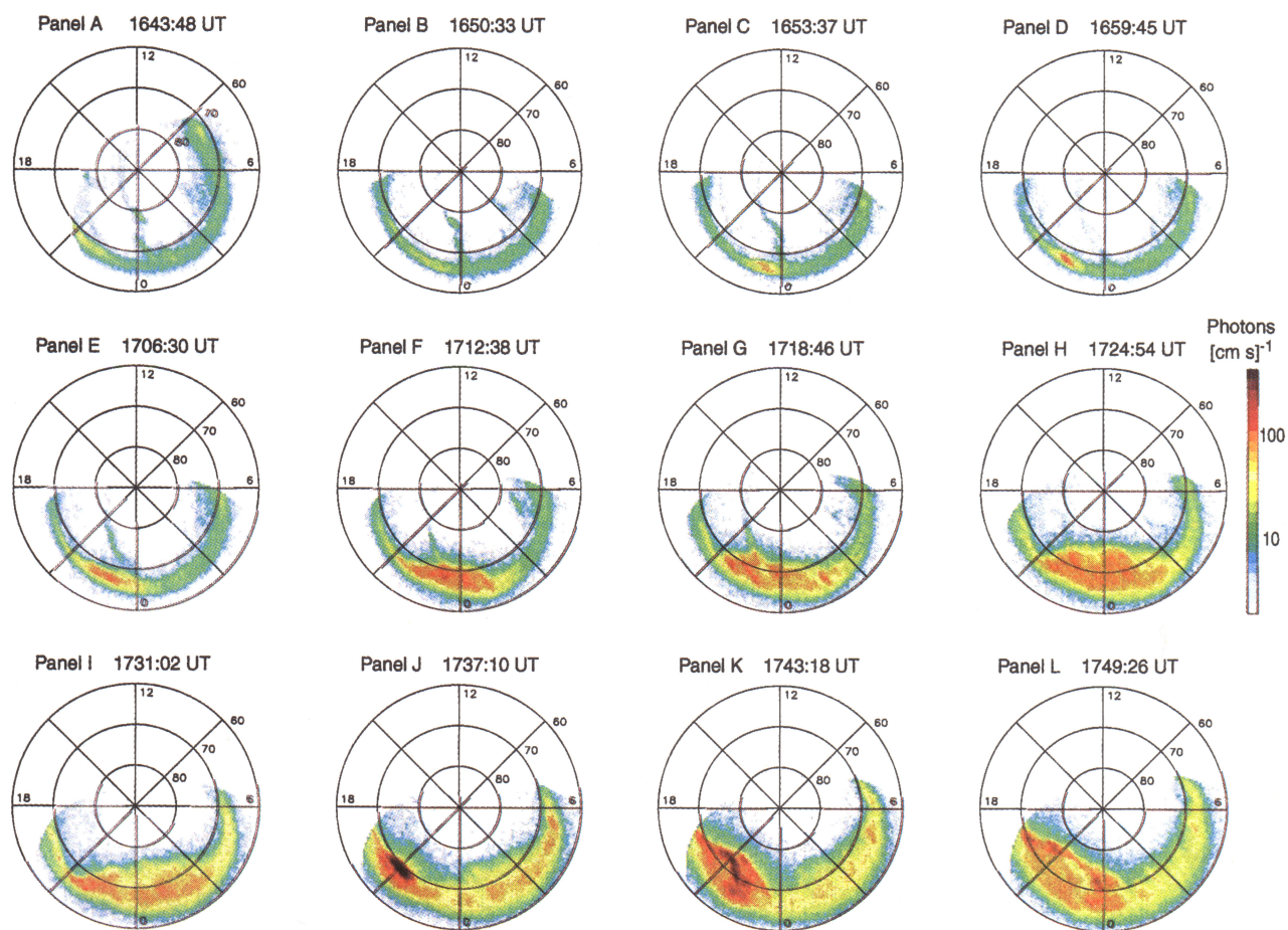
Plate 3. Sequence of 12 global UV images during the event labeled the center time of 37 s exposure time. The images show the response in the LHBL band where the emissions are primarily created by the electron impact on \text{N}_2 . The first onset is seen in Plate 3e, while the second, more intense breakup further west is seen in Plate 3j. Note that a logarithmic scale and CGM grid have been used.
