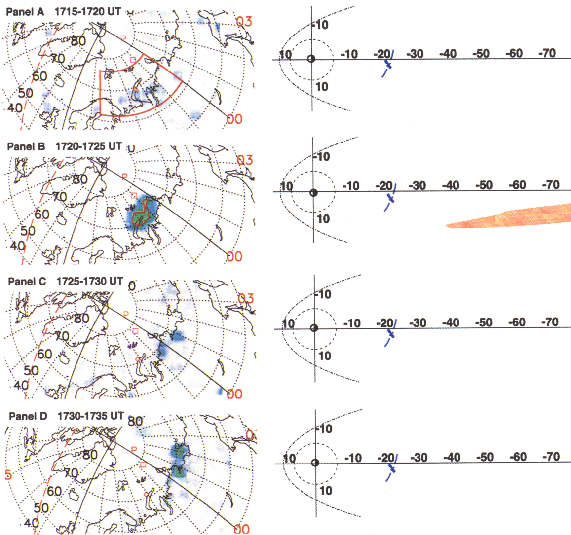
Plate 2. (left) X-ray images from the PIXIE instrument; (right) corresponding source areas (of the red contour) in the magnetosphere. Each PIXIE image in this sequence represents a 5-min accumulation of the X-ray flux within the given time interval. The grid is CGM coordinates. Local time is labeled with red numbers. The source areas are mapped using the Tsyganenko T96 magnetic field model, parameterized with realistic solar wind input parameters. The reference area used for calculation of the area integrated differential fluxes is marked in Plate 2a. (e-h) Note that the mapping now places Geotail spacecraft within the source area, a view also supported by the measurements from Geotail.
