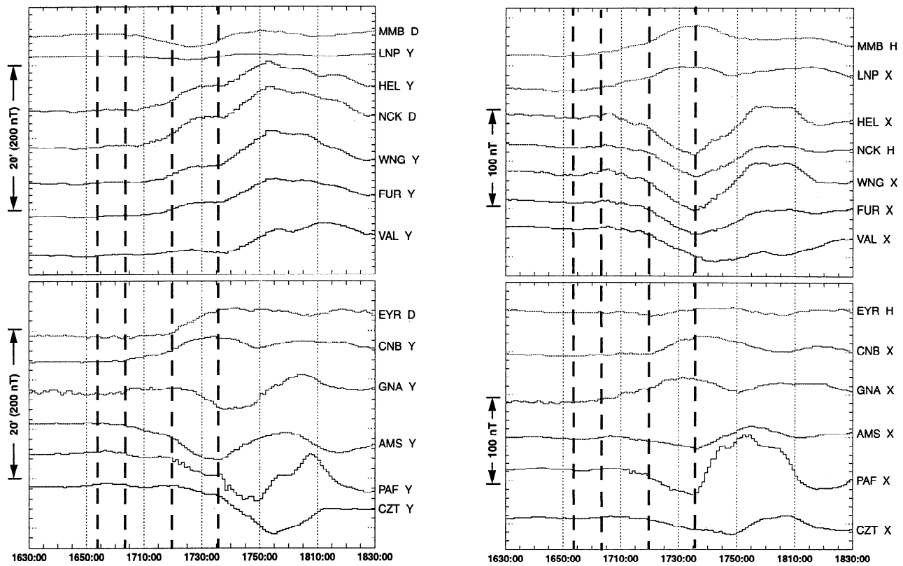
Figure 4. (left) East-west components of the ground magnetic field from selected stations in the northern hemisphere (top part of the plot) and the southern hemisphere (bottom part of the plot). (right) Horizontal components from the same set of stations. Note that some of the stations use a HDZ system where the east-west deflection is given in degrees, while the other stations use a XYZ coordinate system. The first reconnection signature at Geotail at 1654 UT, the onsets at 1704 and 1736 UT and the transient increase of energetic precipitation at 1720 UT are marked with dashed lines. Full names and CGM coordinates of the stations are given in Table 1. The locations of the stations are also indicated in Figure 5.
