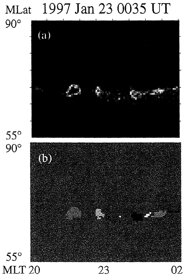
Figure 2. Analysis of an auroral image from Polar: (a) auroral distribution is transformed into coordinates of MLat and MLT, (b) identification of individual auroral activity region.
