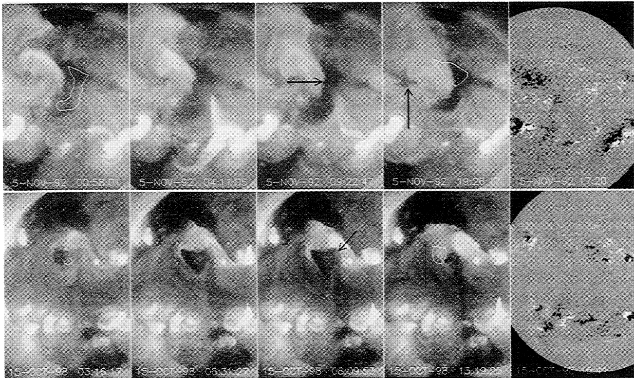
Figure 1. (top) Al filter Soft X-ray Telescope (SXT) images showing a pair of transient coronal holes (TCHs) forming near a bend in the magnetic neutral line (NL) as an arcade developed along a northeast-southwest NL on November 5, 1992. The large positive polarity TCH developed adjacent to a small midlatitude coronal hole, and a small negative polarity TCH, shown by the arrow in the 1926 UT image, developed to the east. The arcade boundaries, one of which is shown by the black arrow in the 0922 UT image, advanced into the areas of the TCHs throughout the event. Initially, the outer boundary of the western TCH receded (0411 UT), but then also contracted (0922, 1926 UT). The contour lines show the TCH boundaries at the times of the first and last images, interchanged, for reference. The last image is the Kitt Peak National Observatory (KPNO) magnetogram with positive and negative polarities shown as white and black, respectively. (bottom) AlMg filter SXT images showing a large TCH forming in a negative polarity field region south of a bend in the NL on October 15, 1998. The arcade boundary shown by the black arrow on the 0809 UT image expanded into the TCH from the north as the loop system lying parallel to the southern boundary receded away from the NL. Loop brightening in the south and arcade expansion in the north then forced the TCH boundaries to contract to a small area at 1319 UT. The last image is the KPNO magnetogram with positive and negative polarities shown as white and black, respectively.
