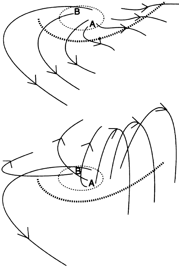
Figure 3. Cartoon showing a suggested configuration leading to the formation of a transient coronal hole (TCH). The dashed line is a magnetic neutral line (NL) with a curve, or bend. (top) The magnetic field lines of the TCH are connected to a larger area of weaker fields on the opposite side of the NL. As the strongly sheared fields erupt along the NL, those TCH fields from region A extending into the sheared region also erupt. (bottom) As the post-eruptive arcade forms, the first TCH fields to open are closed in the reconnection process. At the same time, the fields of the farther region B of the TCH proceed to open and increase the TCH area.
