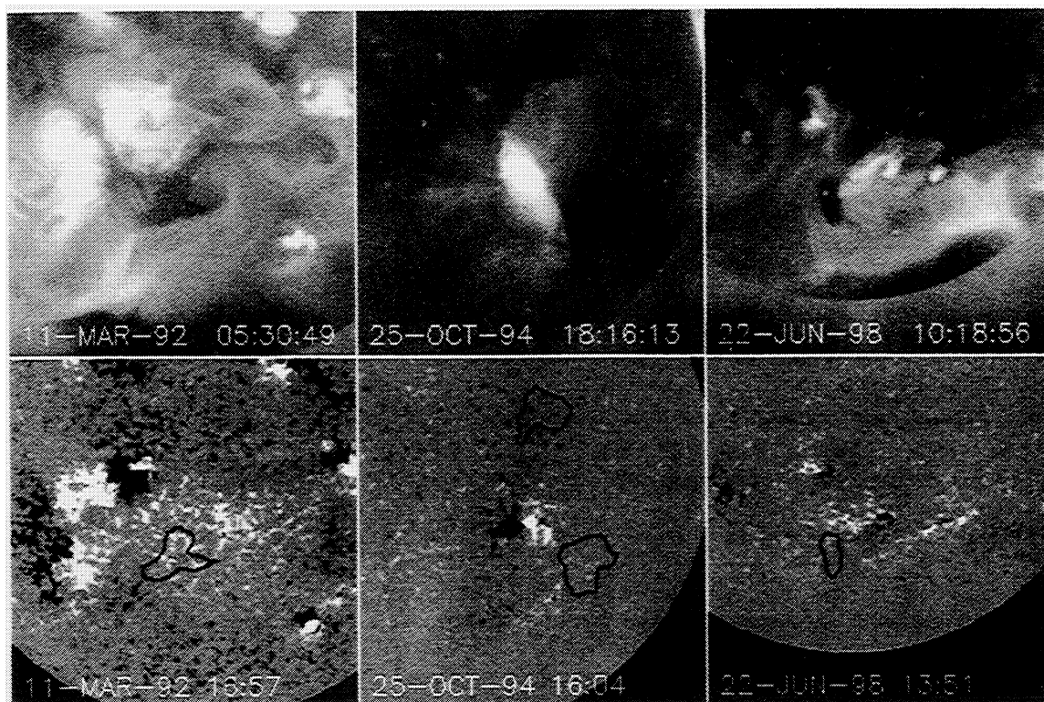
Figure 2. Three comparisons between TCHs and aligned KPNO magnetograms. Lines on the latter indicate approximate TCH boundaries. (left) March 11, 1992. The TCH lies in an area of strong positive fields north of an extended east-west NL where the arcade forms. (middle) October 25, 1994. The northern TCH lies in a negative polarity region along a bend of the NL to the northwest from AR 7792. The southern TCH is characterized by somewhat stronger fields than those across the north-south NL. (right) June 22, 1998. The TCH lies in a positive polarity region adjacent to the trailing positive polarity fields of AR 9049.
