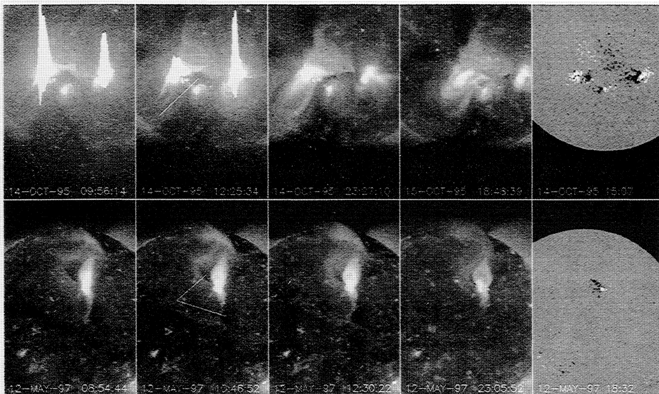
Figure 4. (top row) AlMg SXT images and KPNO magnetogram. The TCH of October 14, 1995, lies in a weak negative polarity region surrounded by the negative polarity fields of AR 7912 in the east and AR 7910 in the west (the diagonal line in the second panel shows the location). AR 7913 lies south of the TCH. The initiation of the TCH follows a flare in AR 7912. The developing arcade along the NL northwest of AR 7912 and loops from AR 7913 expand into the TCH, causing the TCH area to vanish on October 15. (bottom row) Al.1 SXT images and KPNO magnetogram. The two TCHs of May 12, 1997, indicated by the lines, lie in a weak negative polarity region in the north and a weak positive polarity region in the south. The arcade extends to the north of the northern TCH along a bend of the NL to the northeast. The more easily observed northern TCH has vanished by 2305 UT.
