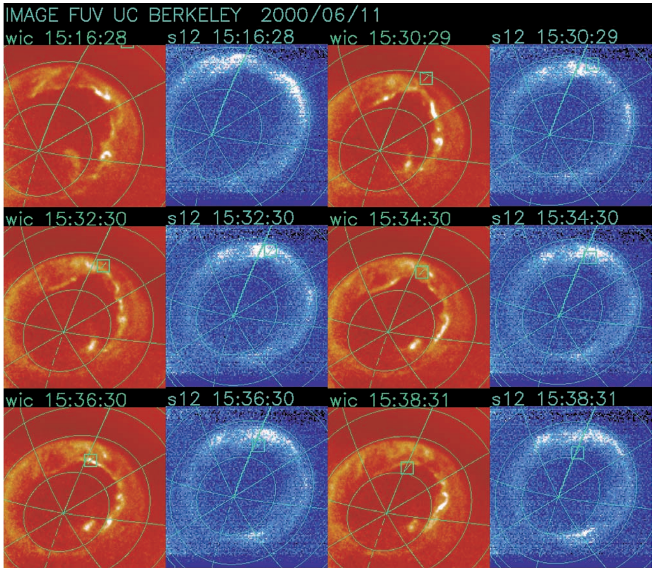
Figure 1. Collage of simultaneous WIC and SI12 images with superimposed geomagnetic latitude (45, 60, 75 and 90) and magnetic local time (midnight, 0300, 0600, 0900, 1500, 1800, 2100) green solid lines, and magnetic midday with dashed line.
