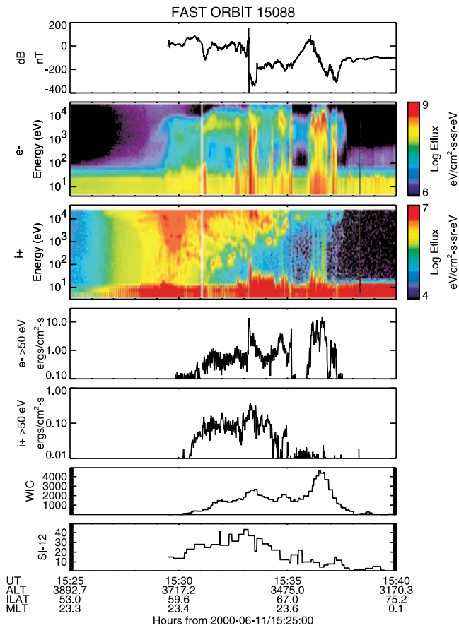
Figure 2. Fast data for the overpass shown in Figure 1. Panels are magnetic field, Downward (pitch angle 0–30) electron energy flux spectrogram, downward proton energy flux spectrogram, electron energy flux, ion energy flux, WIC counts and SI-12 counts.
