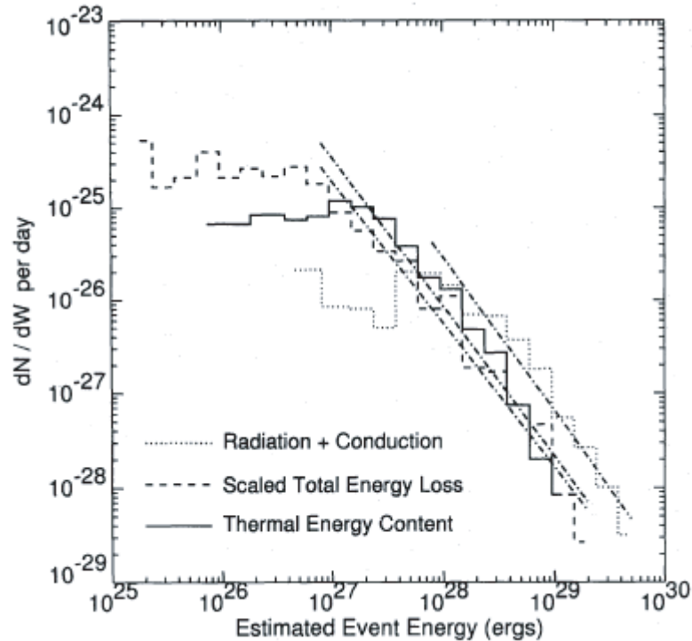
Figure 8.7. Energy distributions for microflares observed with the Yohkoh SXT (Shimizu 1995), incorporating plausible physical models to scale the total energy. The flattening of the distribution for small event energies represents detection threshold.
