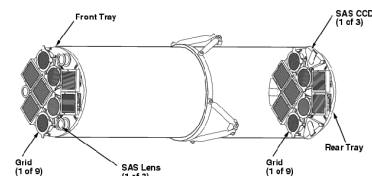
Figure 1. Sketch of RHESSI. The X-ray/ \gamma -ray imager points to the left, and the two sets of grids form nine rotating modulation collimators. The SAS instrument essentially of three lenses on the front grid tray and three linear CCDs on the rear grid tray.
