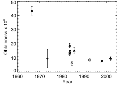
Figure 8. Recent history of solar oblateness measurements.
