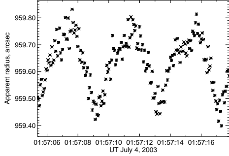
Figure 5. Expanded view of data similar to the Figure 4. One can now see the limiting random error in the data, which amounts to about 30 mas ( 10^{-3} arc sec, roughly parts per million). The cyclical variation of about 300 mas results from coning motions of the RHESSI rotation and can easily be removed.
