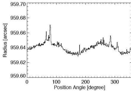
Figure 9. Summation of about three days' data from the stackplot of Figure 6. This shows a clear oblateness signal at about the right amplitude, together with many excess peaks due to faculae at the limb.
