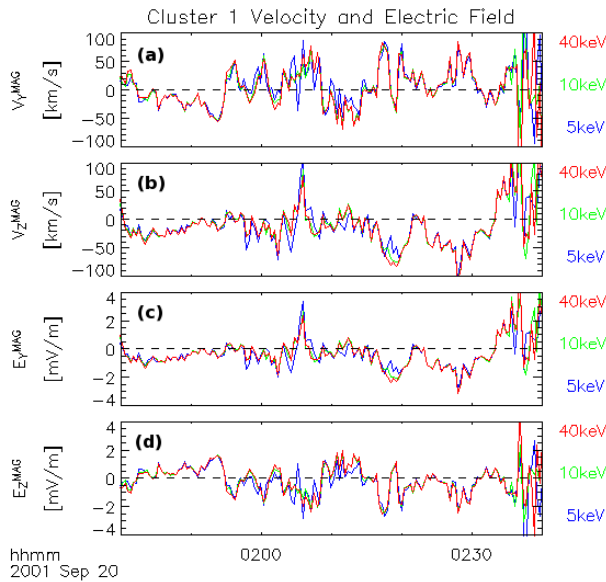
Fig. 9. The Y_{MAG} and Z_{MAG} components of \mathbf{V} (a, b) and \mathbf{E} (c, d), obtained by integration of the 3-D CODIF H^+ distributions from SC1 over three energy ranges, from 40 eV up to 5 keV (blue), 10 keV (green), and 40 keV (red). As for SC1, the results for SC3 and SC4 (not shown) do not exhibit a significant dependence on the upper limit of the energy range.
