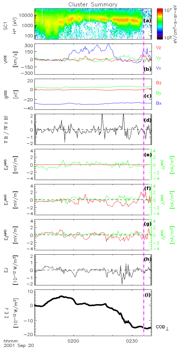
Fig. 7. Summary of Cluster data for the time interval 01:40–02:40: (a) CODIF H^+ energy spectrogram from SC1; average (b) H^+ velocity and (c) magnetic field; (d) normalized divergence of the magnetic field, \nabla \cdot \mathbf{B}/|\nabla \times \mathbf{B}| ; (e–g) components of the electric field, as derived from CODIF data, and current density, in the MAG reference system; (h) \mathbf{E} \cdot \mathbf{J} and (i) its cumulative sum. The velocity, as well as the electric field, are averaged over SC1, SC3, and SC4. The magnetic field is averaged over all spacecraft. The conjunction with FAST is indicated by the vertical magenta line.
