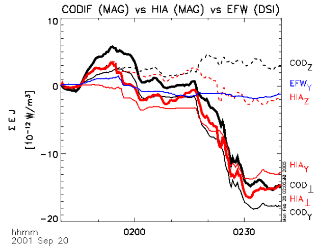
Fig. 10. Cumulative sums of \mathbf{E} \cdot \mathbf{J} , with \mathbf{E} estimated from CODIF (black), HIA (red), and EFW (blue) data. In each case the electric field is averaged over the satellites where the respective instrument is operational. For CODIF and HIA the thick solid lines show the total, while the thin solid and dashed lines indicate the contributions from the Y_{MAG} and Z_{MAG} directions. For EFW only the contribution from the Y_{DSI} direction is shown.
