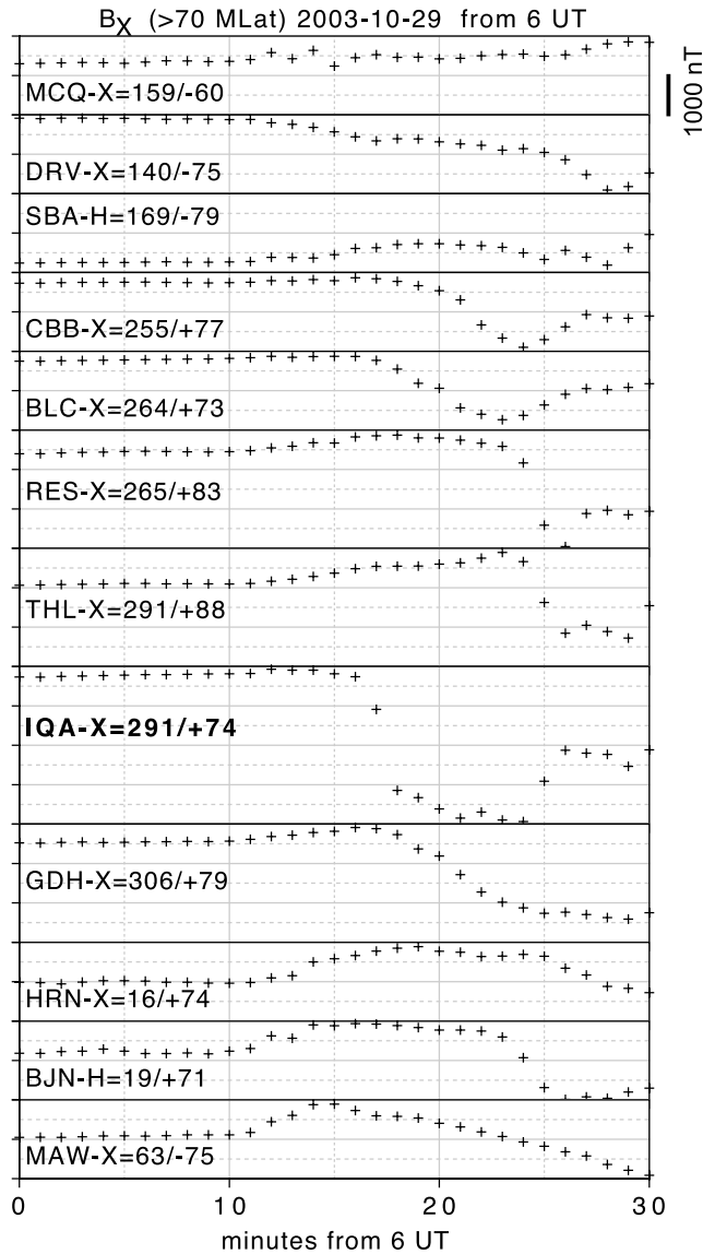
Figure 7c. Worldwide geomagnetic field on 2003-10-29 at 0600–0630 UT in the high latitude side of the auroral zone (GMLat > 70°).
