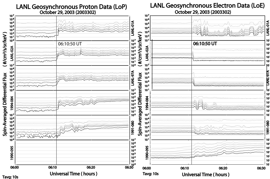
Figure 3. Energetic particle data from the SOPA instrument on board the LANL geosynchronous satellites during the initial phase of the 2003-10-29 storm (0600–0630 UT). (a) Proton flux (50–400 keV); (b) electron flux (50–300 keV). The local times of the satellites at 06 UT are, from top to bottom, 07 LT (LANL-01A), 11 LT (LANL-02A), 13 LT (LANL-97A), 16 LT (1994-084), 19 LT (1991-080), and 04 LT (1990-095).
