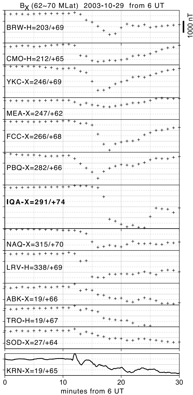
Figure 7a. Worldwide geomagnetic field on 2003-10-29 at 0600–0630 UT in the auroral zone (GMLat \approx 65^\circ ).
