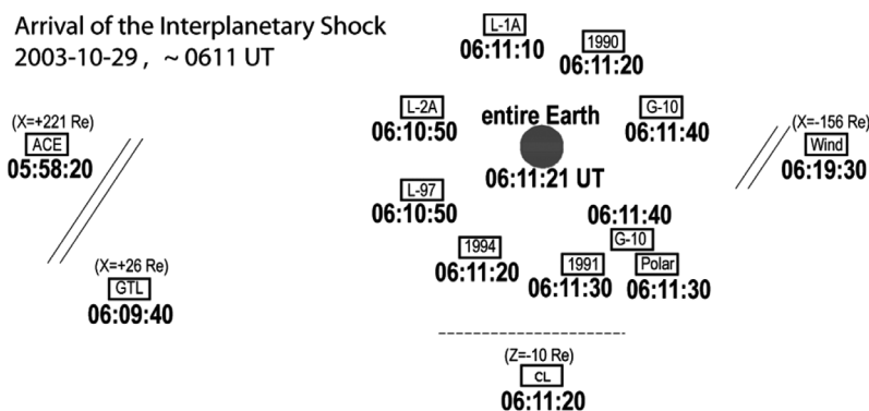
Figure 6. Illustration of the spacecraft locations viewed from the north (except Cluster) at around 0600 UT on 2003-10-29 when the interplanetary shock passed the Earth. Shock was registered in the magnetometer data of ACE, Geotail (GTL: 1-s resolution), and Wind spacecraft in the solar wind and Cluster (CL), Polar (PLR), GOES (G) satellites inside the magnetosphere. The energetic particles data by LANL satellites, i.e., LANL-01A (L-1A), LANL-02A (L-2A), LANL-97A (L-97), 1994-084 (1994), 1991-080 (1991), and 1990-095 (1990) also show the shock arrival. Time resolution is 10 s or better except for ACE (16-s resolution).
