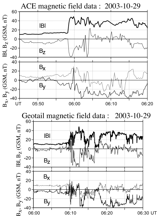
Figure 2. Interplanetary magnetic field data observed before and after the strong interplanetary shock that caused the sudden commencement of the geomagnetic storm at around 0610 UT on 2003-10-29. (a) ACE spacecraft (221 R_E upstream) with 16-s resolution, (b) Geotail spacecraft (26 R_E upstream) with 1-s resolution.
