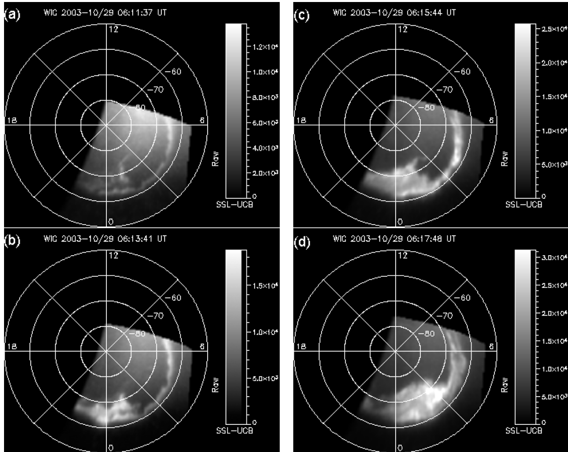
Figure 8. IMAGE-FUV data in the magnetic coordinate (GMLat and MLT) at 0611–0618 UT on 2003-10-29 taken from the southern hemisphere: (a) at around 0611:40 UT; (b) at around 0613:40 UT; (c) at around 0615:40 UT; (d) at around 0617:40 UT.
