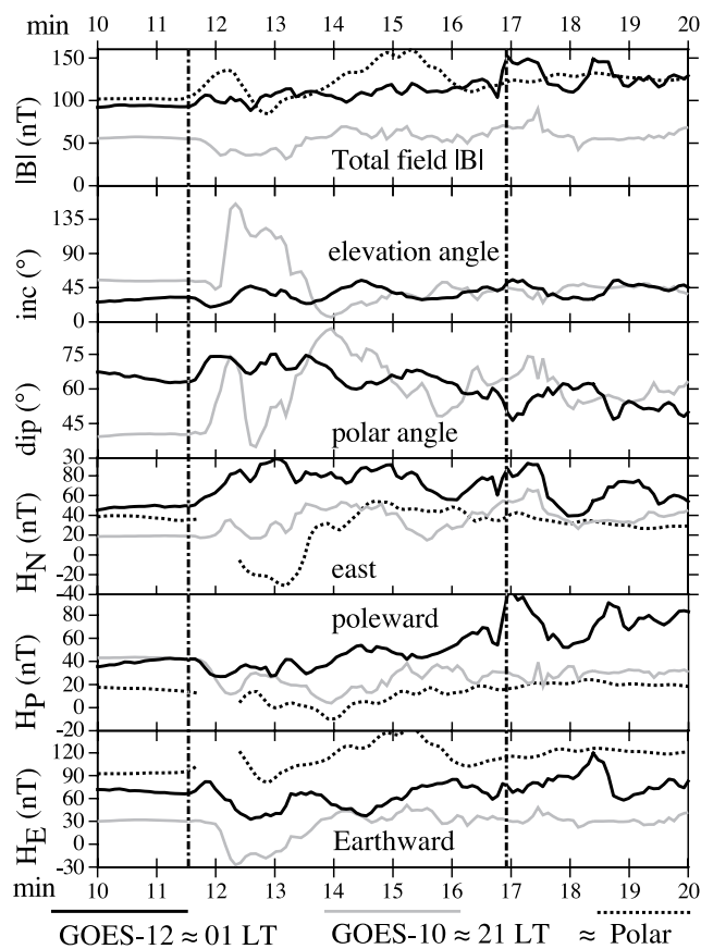
Figure 4. Magnetic field data (5-s resolution) from geosynchronous GOES-10 at around 21 LT (thin lines) and GOES-12 at around 01 LT (thick lines) during the initial phase of the 2003-10-29 storm (0610–0620 UT). H_P is northward component perpendicular to the spin plane (nearly parallel to the Earth's spin axis); H_E is Earthward component perpendicular to H_P ; H_N is eastward component completing local Cartesian coordinate; |B| is total field; \text{inc} = \text{atan}(H_P/H_E) ; and \text{dip} = \text{acos}(H_P/|B|) . Magnetic field data from Polar (6-s resolution), which was located only 1 R_E away from GOES-10 at 21 LT, is overplotted with broken lines in the SM coordinate system ( H_P : parallel to Earth's dipole axis and 11^\circ off from Earth's spin axis). The vertical dot-dashed lines (0611:40 UT and 0616:40 UT) indicate the arrival time of the shock and the onset timing of the very localized 4000 nT activity at the ground (see section 3.1), respectively.
