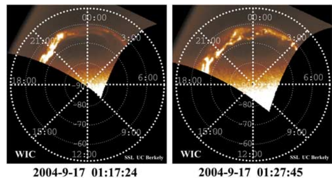
Figure 2. Auroral brightening observed by IMAGE/WIC in the event of 17 September 2004.
