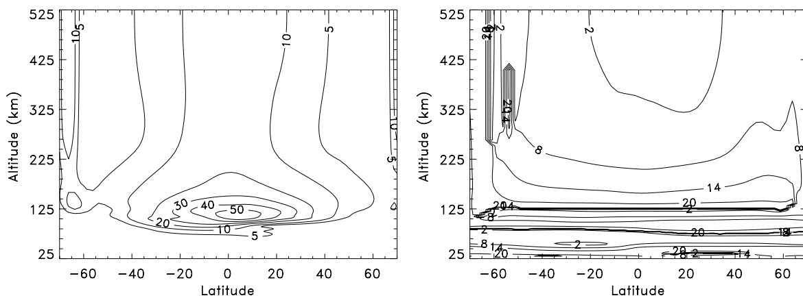
Figure 4. (left) Zonal wind amplitude (m/s) and (right) phase (local solar hours at 0° longitude) of the eastward propagating zonal wavenumber-3 diurnal tide versus latitude between 70°S and 70°N and altitude (km) from the TIME-GCM standard IGRF model run.
