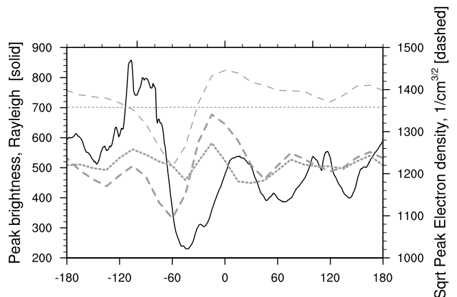
Figure 3. The square root of peak electron density at 2000 Solar Local Time between 0^\circ and 45^\circ\text{N} and 250 and 500 km versus longitude for the TIME-GCM standard model run with (thick long dash) and without tropospheric tides (thin long dash) and for the aligned dipole field with (thick dot) and without (thin dot) tropospheric tides along with IMAGE-FUV peak brightness measurements (solid) after Immel et al. [2006].
