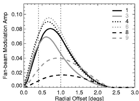
FIG. 2. The fitted amplitude of the fan-beam modulation (for a uniform solar disk) as a function of radial offset from the target. The modulation is maximized at offsets from 0.4^\circ to 1.0^\circ .
