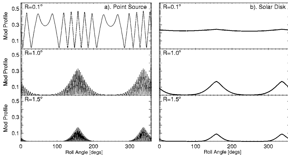
FIG. 1. The expected modulation profile of (a) a point source and (b) the solar disk through one of RHESSI's rotating collimators, for three different radial offsets between RHESSI pointing and source center. Normal RHESSI imaging is based on the rapid modulation in the left panel.
