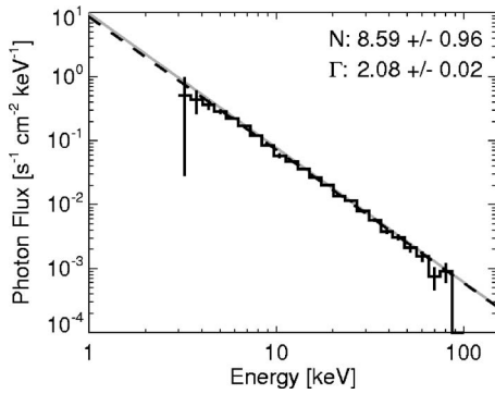
FIG. 8. The spectrum of the Crab found using the fan-beam modulation technique (histogram). The dashed black line is a power-law fit to the data between 4 and 60 keV. The gray line is the reference spectrum from Toor and Seward (Ref. 8).
