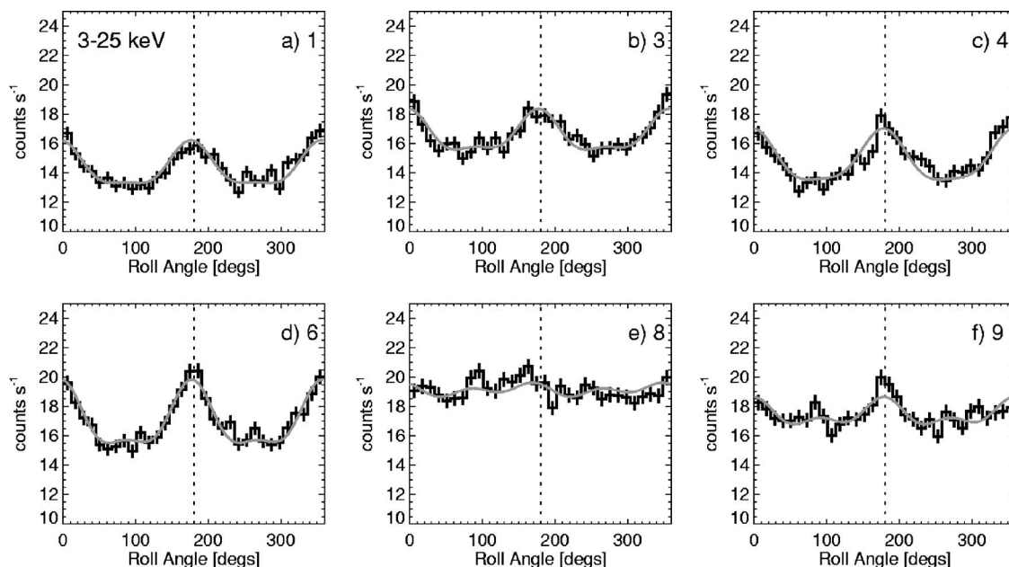
FIG. 7. The stacked 3–25 keV RHESSI counts for an hour-long integration during Crab offpointing in June 2004. The roll angle has been corrected for the orientation of the grids and relative positions of the Crab and RHESSI pointing, so that the Crab signal should be at 0^\circ and 180^\circ . The continuous line shows the model fit for a point source at the location of the Crab Nebula. These data have not been corrected for grid-dependent parameters such as thickness.
