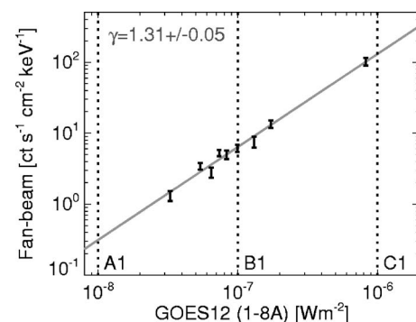
FIG. 5. The mean counts flux in 4–6 keV obtained using the fan-beam modulation technique for nine microflares occurring during quiet Sun offpointing, compared to the background subtracted GOES 1–8 Å flux.
