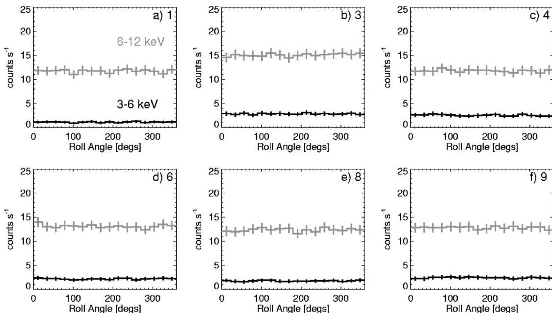
FIG. 9. The stacked RHESSI counts through each suitable subcollimator for 1 h of quiet Sun during offpointing. Two energy bands are shown: 3–6 keV (black) and 6–12 keV (gray). Note that the roll angle has been corrected for the orientation of the grids and relative positions of the Sun and RHESSI pointing, so that the solar signal should be at 0^\circ and 180^\circ
