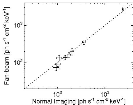
FIG. 6. Comparison of the mean 4–6 keV photon flux, obtained using the fan-beam modulation technique, and the photon flux found through a normal RMC9 back-projection image, for eight microflares (imaging was not possible for one of the nine microflares shown in Fig. 5).
