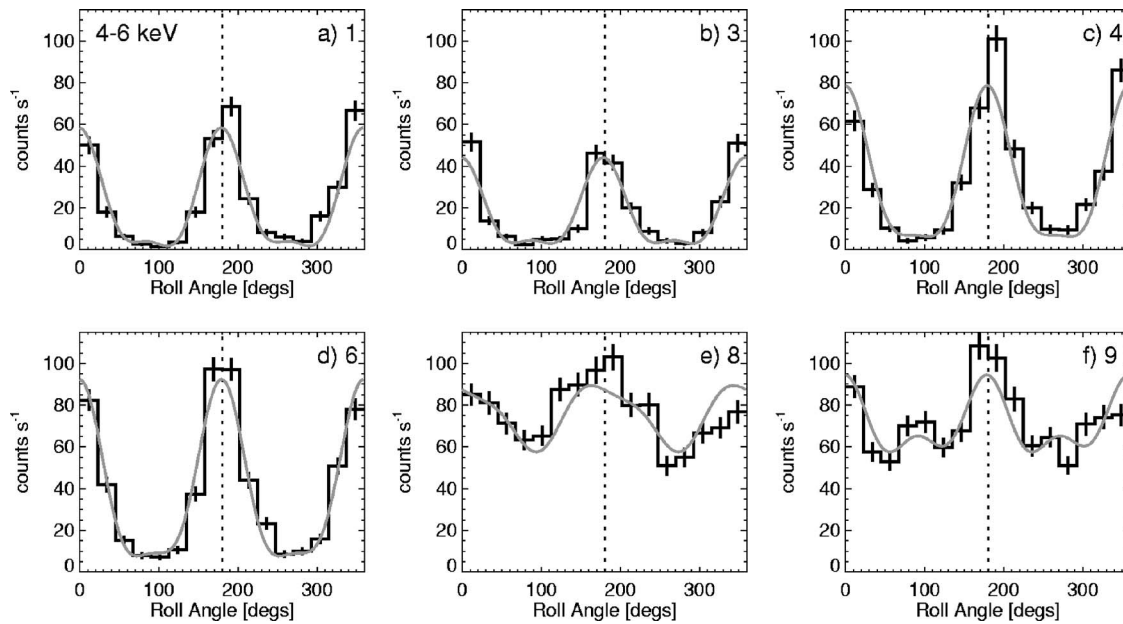
FIG. 4. The stacked RHESSI counts in 4–6 keV through each suitable subcollimator for an A8.3 microflare. In this fit we have included the first harmonic as well as the fundamental term. Since the roll angle has been corrected for the orientation of the grids and relative positions of RHESSI pointing and the microflare, the signal should peak at 0^\circ and 180^\circ .
