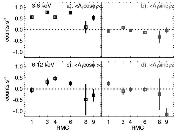
FIG. 10. The mean value of the fit components A_1 \cos \phi_1 [left panels (a) and (c)] and A_1 \sin \phi_1 [right panels (b) and (d)] for detectors RMCs 1, 3, 4, 6, 8, and 9, averaged over the 1522 5-min quiet Sun time intervals. The top row shows the results for 3–6 keV, the bottom row for 6–12 keV.
