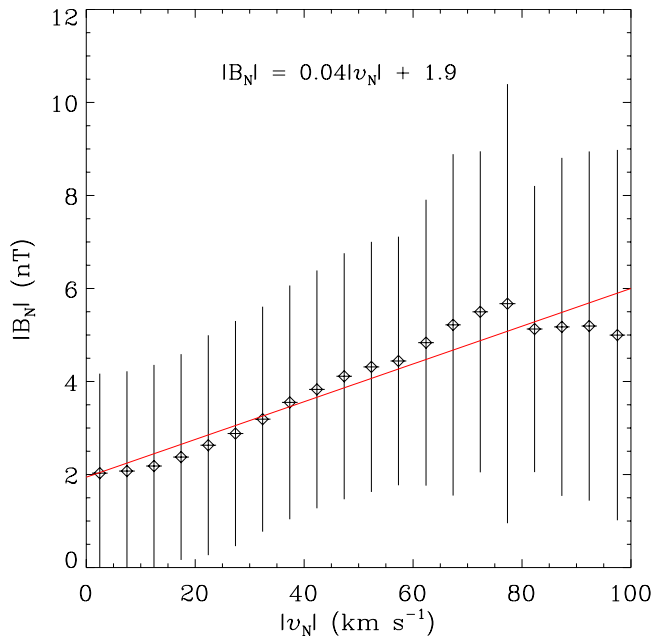
Figure 5. Solar wind meridional field magnitude as a function of the meridional speed. The horizontal and vertical bars indicate the standard deviations of the meridional speed and field within the bins, respectively. Also shown are the best fit of the data (solid line) and the fit parameters (text). Only the normal solar wind is included, as restricted by 0.9 \leq T_p/T_{ex} \leq 1.1 .
