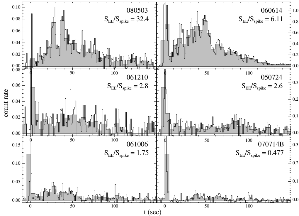
Figure 2. BAT 25–100 keV light curves of several different Swift short bursts with high signal-to-noise ratio extended emission, including GRB 080503 (top left), showing the similar morphology of these events. The 1 s binned curve is plotted as a black line; a 5 s binning is plotted in solid gray to more clearly show the longer-duration extended emission which for most events is near the detection threshold. Possible short GRB 060614 is also shown; it appears very similar to GRB 080503 except that the initial pulse is significantly longer.
