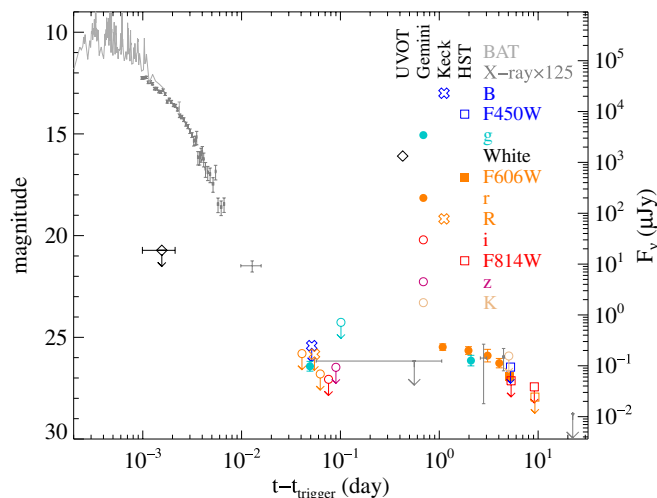
Figure 6. X-ray and optical light curves of GRB 080503. The optical bands have been shifted to the r band assuming an optical spectral index of \beta = 1.2 ; the X-ray light curve has been shifted by a factor of 125 to match the optical (corresponding to \beta_{OX} = 0.75 ). The BAT light curve is extrapolated into the X-ray band using the high-energy spectrum. 3\sigma upper limits are shown with arrows.
