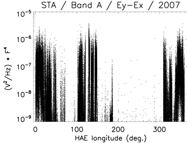
Figure 4. Average power observed by the STEREO/WAVES low frequency receiver ( V_f^2 in \text{V}^2\text{Hz}^{-1} , normalised to f_{\text{kHz}}^4 and integrated in the lower band) on STEREO A as a function of ecliptic longitude during the whole 2007 orbit.
