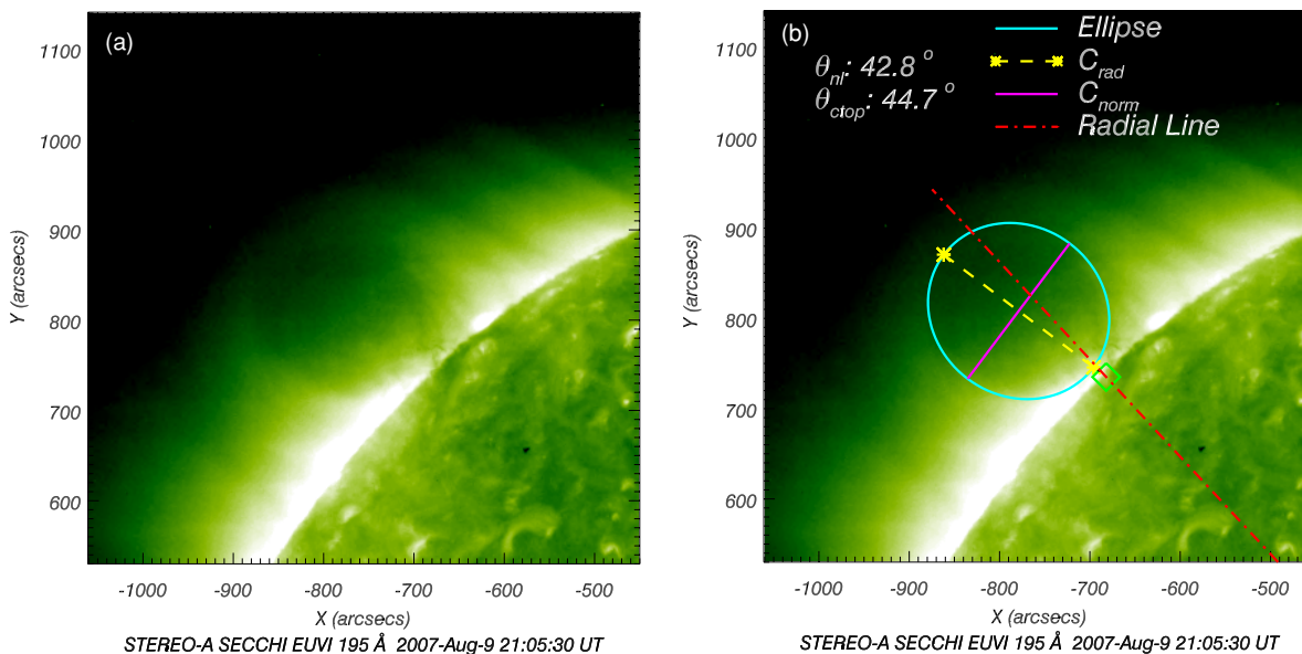
Figure 13. Elliptical fit to the edge of the cavity as observed in EUV. (a) Image from the EUVI-A instrument at 195 Å; (b) we show how an ellipse is fit to user-defined points along the edge of the cavity, providing the input needed to determine model parameters.
