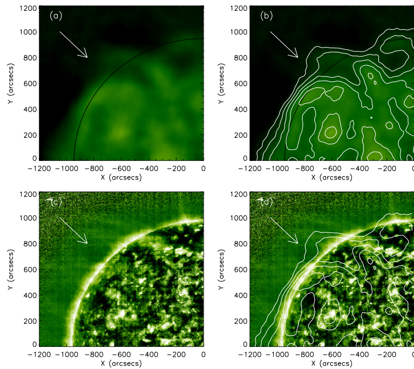
Figure 10. 2007 August 10 observations of the cavity on the NE limb (indicated by white arrow) by (a) Nançay Radioheliograph at 408 MHz (11:30:30 UT) and (c) EIT 195 Å (13:13:46 UT). (b) displays radio isocontours on radio image, and (d) displays radio isocontours on EUV image. Both data sets have been enhanced for better viewing: radio data with a multi-scale filter and EIT data with a local histogram equalization. The solar limb is shown in (a) and (b) as a black line.
