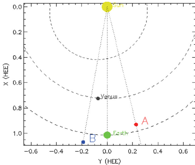
Figure 7. Relative positions of STEREO-B , Earth, and STEREO-A for 21:00 UT 2007 August 9. STEREO-B : east limb Carrington longitude = -37^{\circ}732 , heliographic latitude = 5^{\circ}475 . Earth: east limb Carrington longitude = -27^{\circ}575 , heliographic latitude = 6^{\circ}341 . STEREO-A : east limb Carrington longitude = -13^{\circ}653 , heliographic latitude = 7^{\circ}111 .
