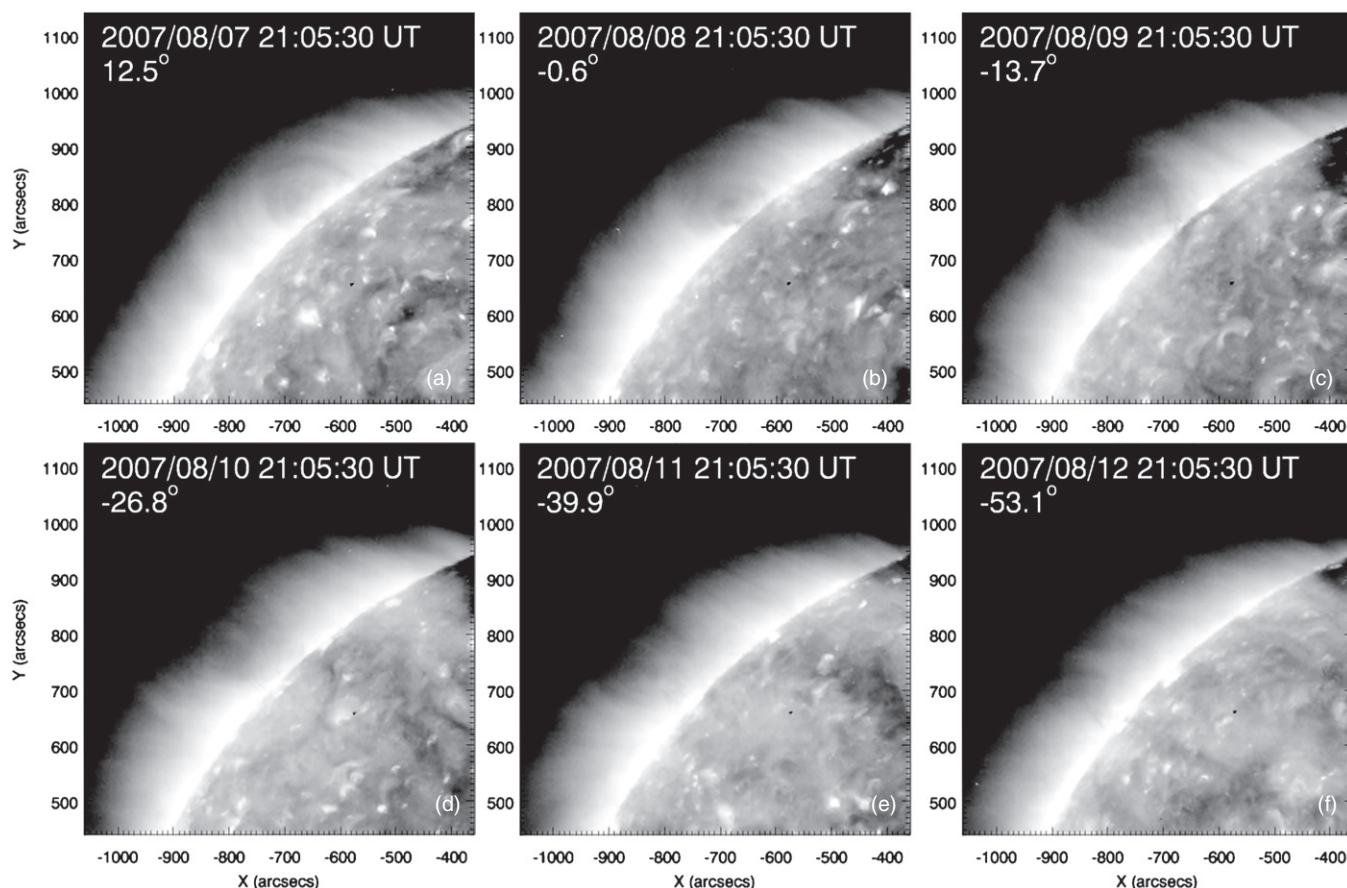
Figure 1. 195 Å images of cavity from STEREO EUVI-A ((a)–(f)) 2007 August 7–12. Numbers below the time stamp indicate Carrington longitude at the east limb on that day ( 90^\circ less than the central meridian Carrington longitude).
