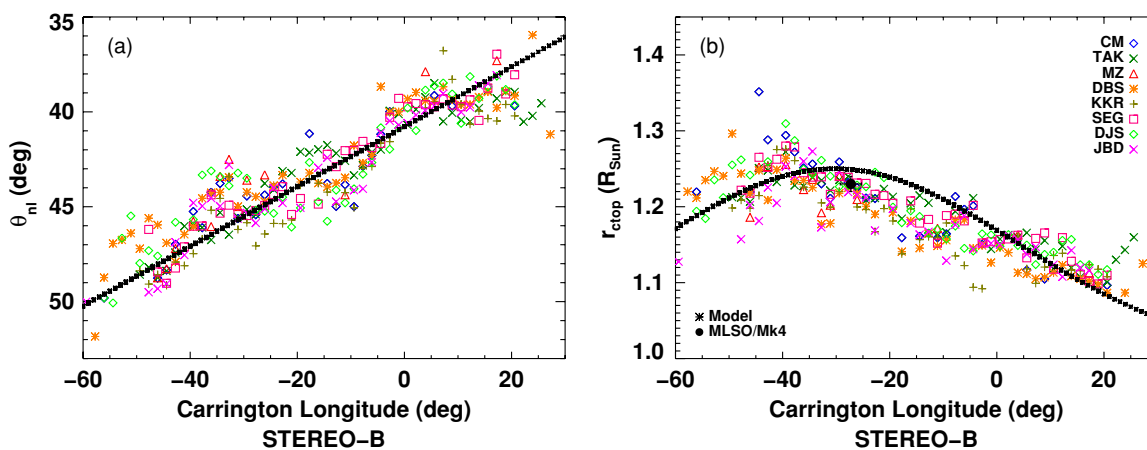
Figure 16. Points based on EUVI-B data plotted with the EUVI-A model fit (black lines) as shown in Figure 14. Standard error for \theta_{nl} is 1\text{:}36 and for r_{ctop} is 0.04 R_{\odot} . We found the quality of data was uniformly better for EUVI-A than for EUVI-B, and so used only EUVI-A data in our fit. (A color version of this figure is available in the online journal.)
