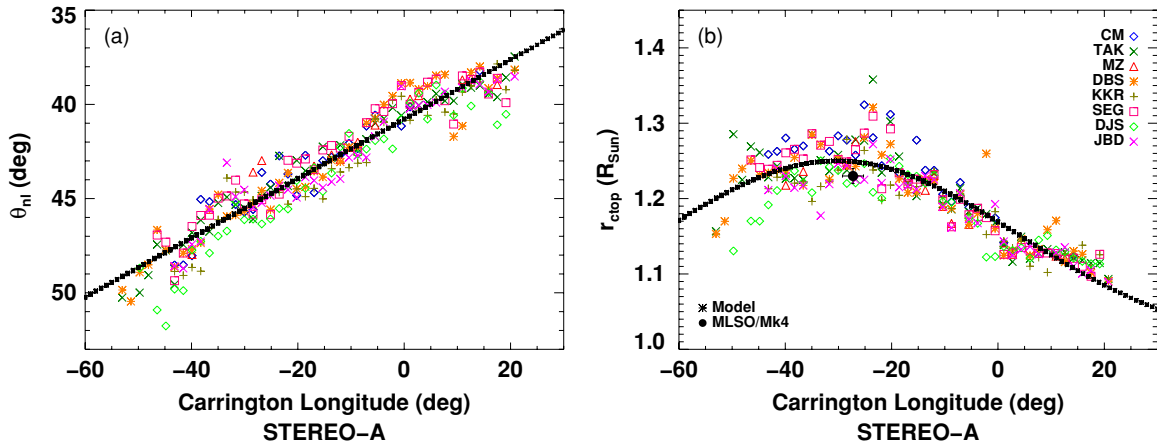
Figure 14. (a) Cavity central colatitude ( \theta_{ni} ) at r = R_{\odot} vs. Carrington longitude, as established by ellipse fits to the cavity as observed in EUVI-A at 195 Å. (b) Cavity top height ( r_{ctop} ) established by same ellipse fits also vs. Carrington longitude. Model fit is shown as black line. Different color/symbol indicates a different co-author doing the fit (identified by initials at right). The large black dot is the location of the cavity top found in white light; see Figure 5(b). Standard error for \theta_{ni} is 1°12 and for r_{ctop} is 0.03 R_{\odot} .
