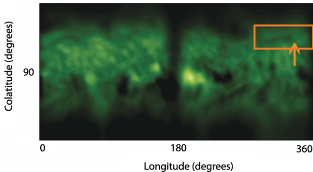
Figure 9. Longitude–colatitude Carrington map (CROT2060) using Nançay Radioheliograph 432 MHz observations taken from a slice at central meridian at an assumed height of 1.025 R_{\odot} (typical value for this frequency). A data gap occurs near map center. The cavity is seen in the orange box; the arrow indicates position to the right of which cavity visibility diminished.
