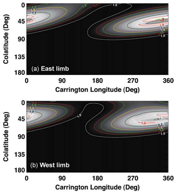
Figure 18. Forward-modeled Carrington map of (line-of-sight integrated) EUV 195 Å emission from the viewpoints of (a) STEREO-A east limb and (b) STEREO-A west limb. Maps from the STEREO-B viewpoints (not plotted) are very similar. Maps show limb emission at the height of the cavity midpoint ( r = 1.125 R_{\odot} ). Contours are in units of \text{DN s}^{-1} .
