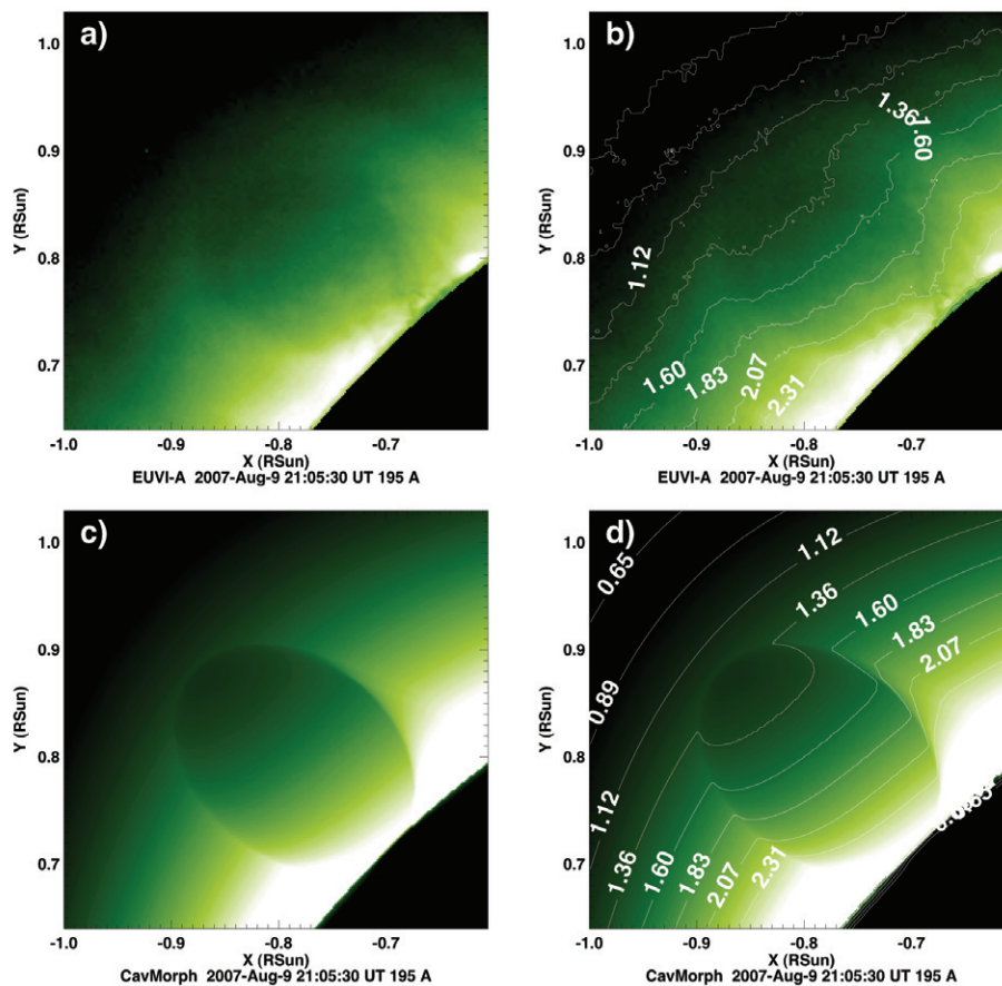
Figure 17. (a) EUVI-A image of the cavity with (b) intensity contours overlaid. (c) Forward-modeled (line-of-sight integrated) EUV emission using model density and temperature with (d) intensity contours overlaid. Contours are in units of \text{DN s}^{-1} . See online movie for a model–data comparison of the variation of cavity location and visibility vs. time/longitude. (A color version and an animation of this figure are available in the online journal.)
