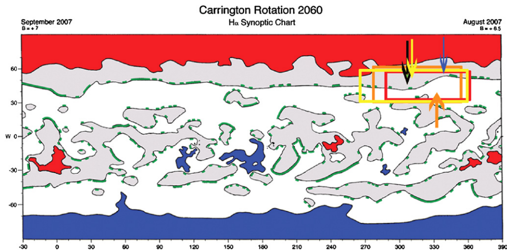
Figure 11. Carrington rotation 2060 ( \pm 30^\circ ) H\alpha synoptic chart (McIntosh 2003). Magnetic polarity is generally indicated by white-positive/gray-negative, with neutral lines shown as black contours. Coronal holes (identified from He -10830\text{\AA} ) magnetic polarity is indicated by blue-positive/red-negative. Filament channels generally lie along neutral lines, with green indicating portions where a filament was observed in H\alpha . The northern PCFC associated with the cavity is clearly visible at all Carrington longitudes. Colored boxes and arrows correspond to those in Figures 8 and 9 (note that the red arrow has been replaced with a black arrow for visibility); blue arrow indicates top of \Lambda -type shape in neutral line (see discussion in Section 4).
