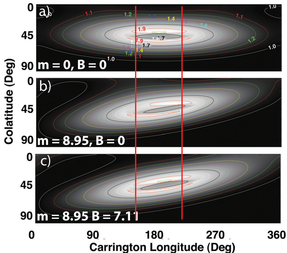
Figure 19. Carrington map (northern hemisphere) of forward-modeled (line-of-sight integrated) EUV 195 Å emission at cavity midpoint height r = 1.125 R_{\odot} . (a) Neutral line angle m and solar B angle set to zero; (b) model value of m , but still has zero B angle; (c) model value of m , and the solar B angle as seen from the viewpoint of STEREO-A during the time of the cavity observations. Note we have shifted to \phi_o = 180 to center the structure for easier viewing. Contours in (a) are in units of \text{DN s}^{-1} ; to avoid cluttering the plot we have not plotted them in (b) and (c), but note that the values for the various color contours are the same in (a)–(c).
