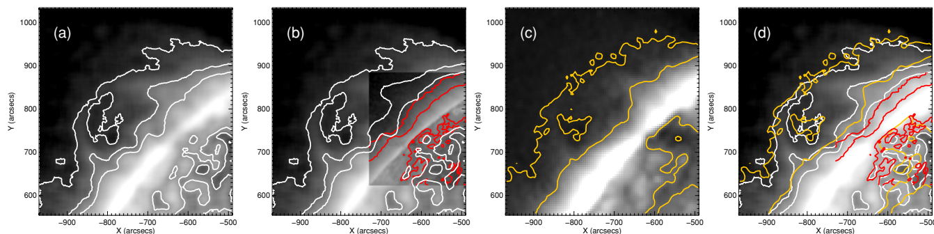
Figure 2. Cavity on 2007 August 9 at a range of wavelengths: (a) SOHO EIT 284 Å, 01:04:50 UT (gray scale and white contours); (b) TRACE 171 Å, 00:01:55 UT (inner image gray scale and red contours) embedded in EIT 284 Å (outer image gray scale and white contours); (c) GOES-SXI , 00:03:06 UT (gray scale and yellow contours); (d) EIT 284 Å (gray scale) with all three contours overlaid.
