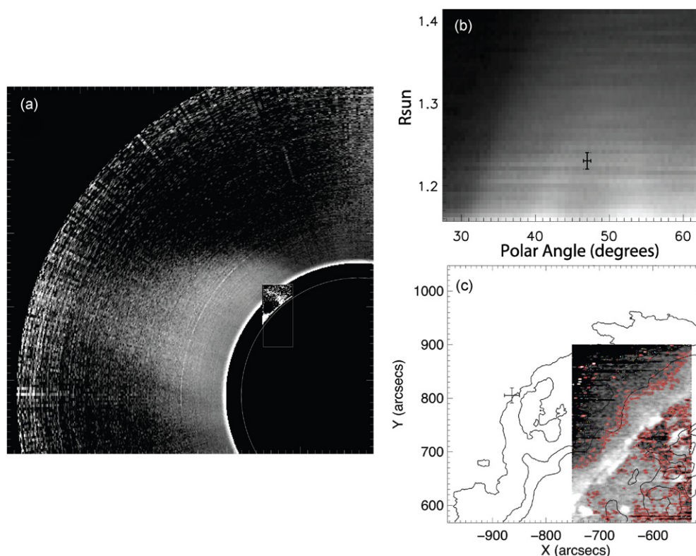
Figure 5. (a) Large-scale white-light streamer surrounding the cavity: MLSO Mk4 white-light (polarized brightness, pB) coronagraph data from 2007 August 9 (19:03:15), and (insert) EIS Fe XII 186/195 Å density-sensitive line ratio from 2007 August 9 (19:46:37). (b) August 9 daily average Mk4 r - \theta pB map of NE streamer and cavity. The error bar brackets the top of the cavity, with a central top height of 1.23 \pm 0.01 R_{\odot} at 47 \pm 0.5 colatitude. (c) Image showing zoomed-in EIS Fe XII 186/195 Å line ratio as a gray scale image indicating depleted density in the cavity (red contours). EIT 284 Å contours and error bar from Mk4 image are overplotted in black.
