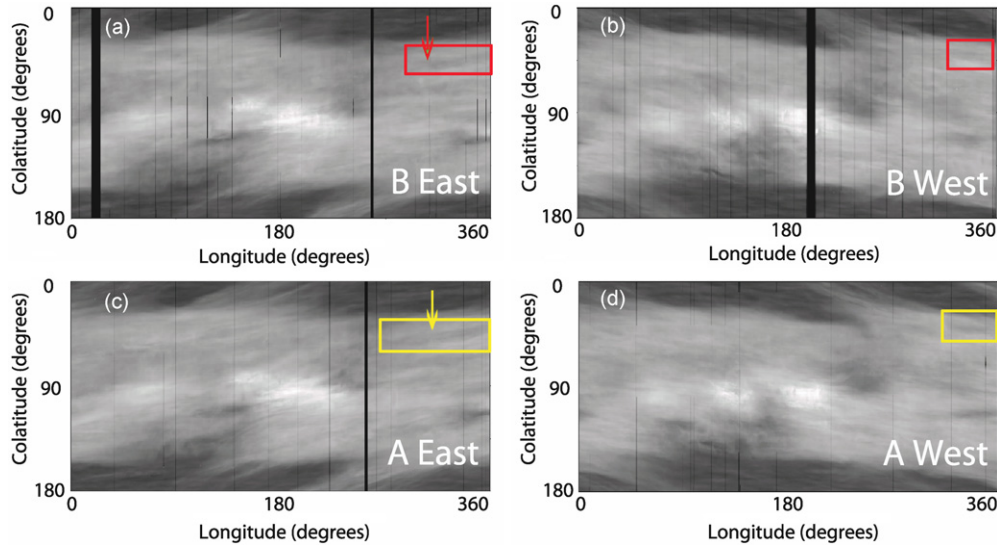
Figure 8. Longitude–colatitude Carrington map (CROT2060) using observations of 195 \text{ \AA} at the solar limb at a height of 1.1 R_{\odot} . (a) EUVI-B east limb; (b) EUVI-B west limb; (c) EUVI-A east limb; (d) EUVI-A west limb. Colored boxes show the location of the cavity observed for each view, which differ both in time and viewing angle. Arrows in (a) and (c) show longitude to the left of which the EUV cavity contrast diminished.
