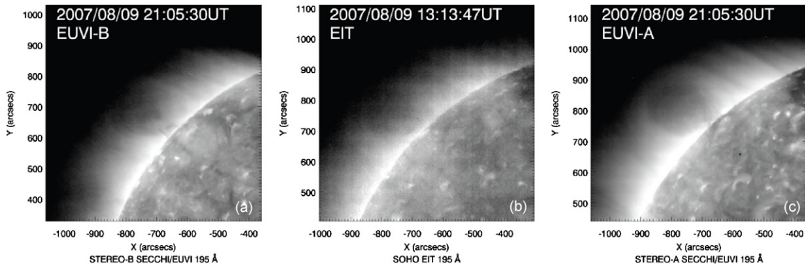
Figure 6. 195 Å images of cavity from (a) EUVI-B, (b) EIT, and (c) EUVI-A.
