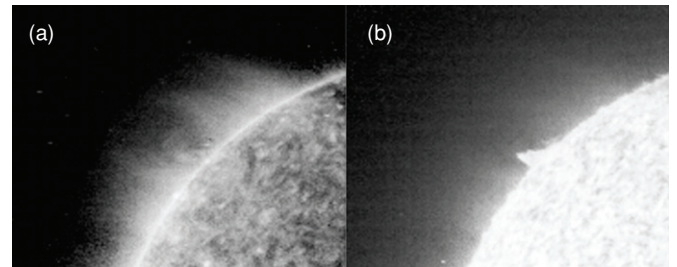
Figure 4. Cavity and associated prominence observed by EIT on 2007 August 10: (a) 284 Å (01:06 UT) and (b) 304 Å (01:19 UT).
