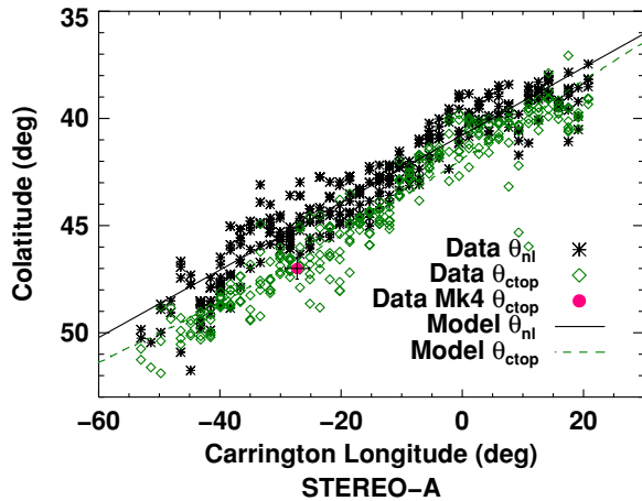
Figure 15. Cavity central colatitude \theta_{ni} (black) vs. cavity top colatitude (green). The red dot shows the colatitude of the cavity top observed in white light. Standard error for \theta_{ni} is 1°12 and for cavity top colatitude is 1°20.
