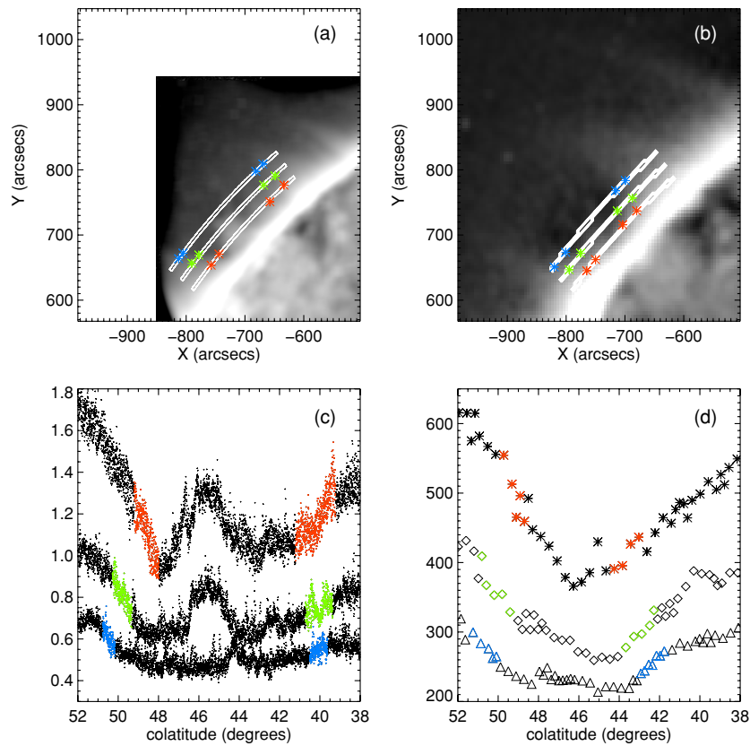
Figure 3. (a) TRACE 171 (August 9, 19:46:20 UT) and (b) SXI (August 10, 00:03:06 UT) observations of the cavity. (c) TRACE 171 intensity vs. colatitude (north pole is to the right) and (d) SXI intensity vs. colatitude corresponding to radial cuts shown in (a) and (b), respectively. Note that increasing radial heights in (a) and (b) correspond to decreasing intensities in (c) and (d). Colored regions indicate edge of cavity determined from images in (a) and (b), with corresponding colatitude ranges indicated in (c) and (d).
