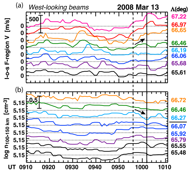
Figure 9. (a) F region I-o-s flow speeds and (b) E region densities versus UT obtained from westward looking beams from 0910 to 1010 UT on 13 March 2008 in the same format as Figure 6.
