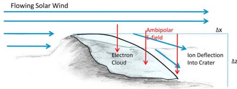
Figure 1. An illustration of the solar wind orographic effect over lunar polar craters. While the solar wind flow is initially horizontal, ambipolar electric fields draw ions into shadowed/solar wind obstructed cratered regions. Thus, ion trajectories are deflected into regions that would be considered “ion-free.” Note the presence of an electron-rich region just leeward of the obstructed flow (called the electron cloud region) where electrons migrate into the void faster than the ions. In a steady state situation, the ions may never fully catch up to the electrons in these regions.
