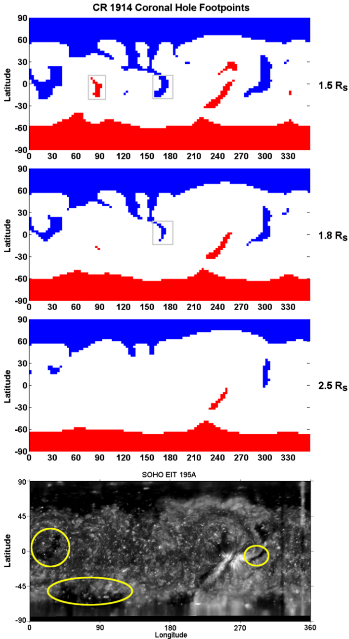
Figure 4 Comparison of PFSS results with 195 \text{ \AA} EUV map for CR 1914 (18 September to 15 October 1996) of cycle 22. For the PFSS modeling, we use solar observations from MWO and source surface heights of 1.5 , 1.8 , and 2.5 R_{\odot} . The yellow circles mark the gross coronal hole features that are largely missing from the 2.5 R_{\odot} mapping results. The gray rectangles mark the gross features that appear in the mapping results but not in the EUV image. The red (blue) areas denote the negative inward (positive outward) field.
