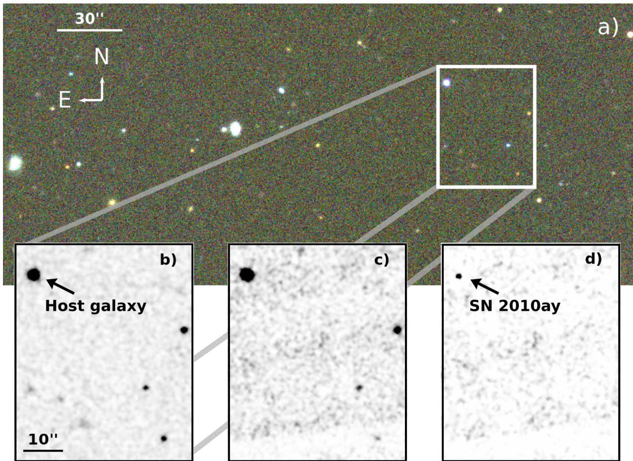
FIG. 1.— Images illustrating the Pan-STARRS1 pre-discovery detection of SN 2010ay and the surrounding field. a) Pre-explosion gri -composite image from the SDSS DR7 (Abazajian et al. 2009), observed 2004 December 21, b) SDSS i -band image geometrically registered to the PS1 image frames and zoomed in to the host galaxy of SN 2010ay, c) i_{P1} -band image from the 3\pi survey of PS1, observed 2010 February 25, d) the difference of the SDSS i' and PS1 i_{P1} images. The transient emission can be seen in the NE corner of the last panel. Nearby stars are included in the zoomed-in frames to illustrate the efficiency of subtraction.
