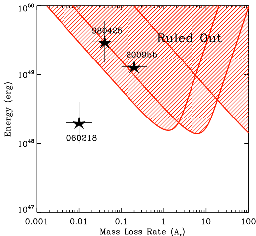
FIG. 7.— The region of energy-mass loss space ruled out (red) by our EVLA observations for on-axis ejecta under the assumption of a free-expansion model.
