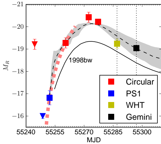
FIG. 2.— The optical R-band light curve of SN 2010ay, as compiled in Table 2 from CBET 2224 (red squares), the PS1 3\pi survey (blue), our Gemini images (black), and synthetic photometry (§2.3) based on our WHT spectrum (gold). Triangles denote upper limits. The thick dashed line represents the luminosity of an expanding fireball fit to our early-time photometry (§3.1). The thin dashed line is the SN Ib/c light-curve template of Drout et al. (2011) and the gray field represents the standard deviation among its constituent photometry. The template is stretched by (1+z) = 1.067 with the best fit parameters t_{Rpeak} = \text{March}18 \pm 2 (MJD 55273 \pm 2 ), M_{Rpeak} = -20.2 \pm 0.2 mag. The solid line is the light-curve of the GRB-SN 1998bw (Galama et al. 1998), redshifted to match SN 2010ay. The vertical dotted lines mark the epochs of our Gemini and WHT spectroscopy.
