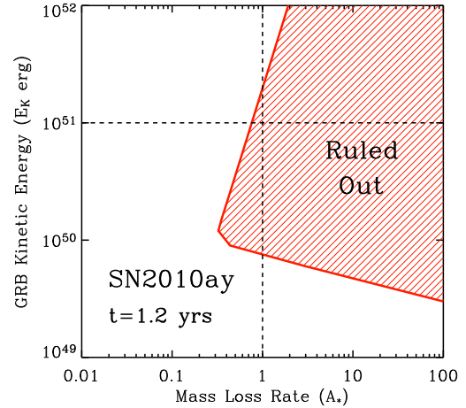
FIG. 8.— Our EVLA observations at \Delta t \approx 1.2 years after explosion constrain the properties of a possibly associated off-axis GRB jet. Using our semi-analytic model as described in §4.2, we assume partition fractions of \epsilon_e = \epsilon_B = 0.1 , \theta_j = 5 degrees, p = 2.5 , and an off-axis viewing angle of \theta_{oa} = 90 degrees. We are able to exclude the region of E_K - A_* parameter space (red) associated with typical GRBs, i.e. E_K = 10^{51} erg and A_* = 1 (dashed black lines).
