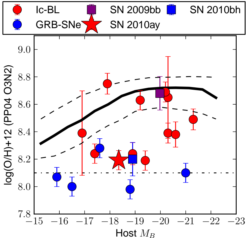
FIG. 9.— A plot of host galaxy metallicity versus absolute B magnitude for SNe Ic-BL (red) and engine-driven explosions (blue). The L-Z relation of nearby starforming galaxies is plotted as a solid line, with the 15th and 85th percentile boundaries of the galaxy distribution (dashed lines). Here we have transformed the k -corrected gri magnitudes from the MPA/JHU catalog to B-band (Blanton & Roweis 2007) and converted the T04 metallicity values to the PP04 scale (Kewley & Ellison 2008), for the purpose of comparing it to metallicity measurements for SN host galaxies in the literature. The host galaxy properties of GRB/SNe other than 2010ay are from the following references: Starling et al. 2011; Cano et al. 2011a (2010bh), Modjaz et al. 2011 (Ic-BL), Levesque et al. 2010d (2009bb), and Levesque et al. 2010a (other GRB-SNe). Errorbars illustrate measurement uncertainty, when published, plus a 0.07 dex systematic uncertainty.
