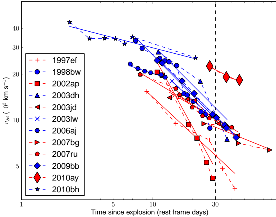
FIG. 5.— A comparison of the time-evolving absorption velocity of SN 2010ay and other SNe Ic-BL (red) and engine-driven explosions (blue) from the literature. For each SN, we fit a power law of the form v_{\text{Si}} = v_{\text{Si}}^{30}(t/30)^\alpha , where t is the time in days, v_{\text{Si}}^{30} is the velocity at 30 days after explosion (dashed vertical line), and \alpha is the velocity gradient. The velocities for SNe 1997ef, 2003dh, 2003lw are from Mazzali et al. (2006), as determined by spectral modeling. The velocities for all other SNe are measured from the Si II \lambda 6355\text{\AA} feature as follows: SN 2007ru are from Sahu et al. (2009); SNe 1998bw, 2006aj, and 2010bh are from Chornock et al. (2010), from spectra in references therein; SN 2007bg are from Young et al. (2010); SNe 2002ap, 2009bb, and 2003jd are from Pignata et al. (2011) and references therein; SN 2010ay is from Prieto (2010) and this paper. See Table 4 for uncertainties.
