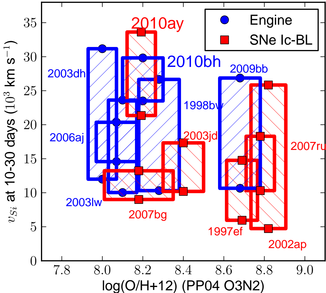
FIG. 10.— SN absorption velocity, as traced by the Si II \lambda 6355\text{\AA} feature, versus host galaxy oxygen abundance for SN 2010ay and other Ic-BL (red) and engine-driven explosions (blue) from the literature (as in Figure 5). The range of velocities hatched for each object comes from the velocity at 10 days and at 30 days after explosion, according to the power law fits presented in Figure 5. The oxygen abundance measurements using the PP04 O3N2 diagnostic are from Levesque et al. (2010a) (GRB-SNe), Sahu et al. (2009) (SN2007ru), Young et al. (2010) (SN 2007bg), and Modjaz et al. (2011) (other SNe Ic-BL). The range of oxygen abundance hatched reflects the error bars quoted in the literature (when stated) plus the \sim 0.07 dex systematic error of the PP04 O3N2 diagnostic (Kewley & Ellison 2008).
