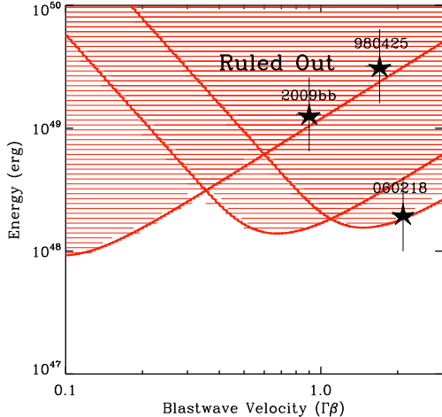
FIG. 6.— The region of energy-velocity space ruled out (red) by our EVLA observations for on-axis ejecta under the assumption of a free-expansion model.
