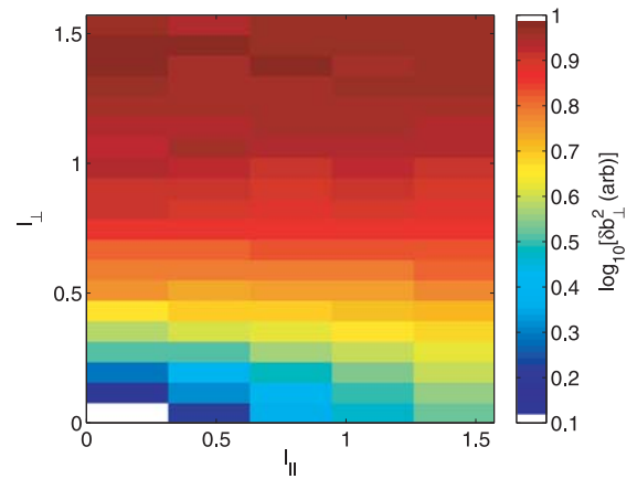
Figure 6. Second-order structure function of the perpendicular magnetic field component for one of the snapshots ( t = 28 ) in the forced simulation as a function of parallel ( l_\parallel ) and perpendicular ( l_\perp ) separation.
