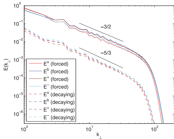
Figure 5. Perpendicular energy spectra of velocity ( E^u ), magnetic field ( E^b ) and Elsasser variables ( E^\pm ) in the forced and decaying periods of the simulation. Slopes of -5/3 and -3/2 are given for reference.
