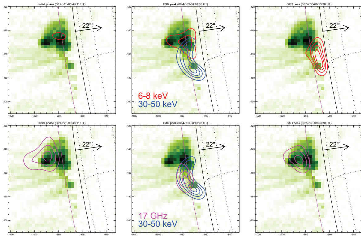
Fig. 4.5 X-ray and microwave imaging during the initial phase of SOL2007-12-31T01:11 (C8.3) (left), the hard X-ray peak (middle), and the soft X-ray peak (right). Top row: Contours in the thermal (6-8 keV, red) and the nonthermal (30-50 keV, blue) range are shown on an EIT 195 Å image taken towards the end of the main hard X-ray peak. The 6-8 keV contour levels are the same for all time intervals at 20, 40, 60, 80% of the maximum emission during the soft X-ray peak time, while the nonthermal emission is shown at 30, 50, 70, 90% levels. Bottom row: Microwave contours (magenta) at 17 GHz are shown at the 50, 70, 90% levels on the same EIT image. For comparison, the 30-50 keV source seen during the impulsive phase is shown as well (blue). The magenta curve gives the location of the limb at 17 GHz, about 12'' above the photosphere; for this reason emission can be seen to lower heights in the HXR images than in the radio images. The black arrows indicate the occultation height for the flare location. From Krucker et al. (2010b).
