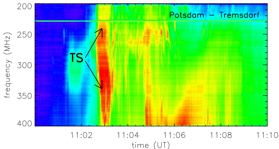
Fig. 7.5 The dynamic spectrum of SOL2003-10-28T11:10 (X17.2), from the Trensford spectrograph operated by the Astrophysikalisches Institut Potsdam. The bright chevron-shaped feature centered at 11:03 UT (labelled “TS”) is identified as a termination-shock feature.
