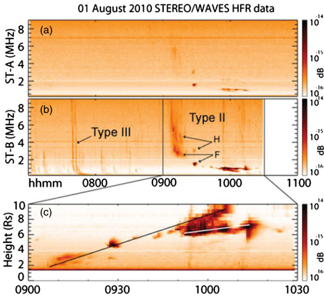
Figure 12. S/WAVES HFR observations from 07:00 to 11:00 UT on 2010 August 1 taken from STEREO-A ( ST-A ; panel (a)) and STEREO-B ( ST-B ; panel (b)) in receiver units and a corresponding time–height plot of a subset of the ST-B data (09:00 to 10:30 UT; panel (c)). The black line in panel (c) indicates the emission generated by CME L (slope 1500 \text{ km s}^{-1} ); the white line appears to correspond to the emission created by the interaction between CME L and CME M (slope 600 \text{ km s}^{-1} ).
