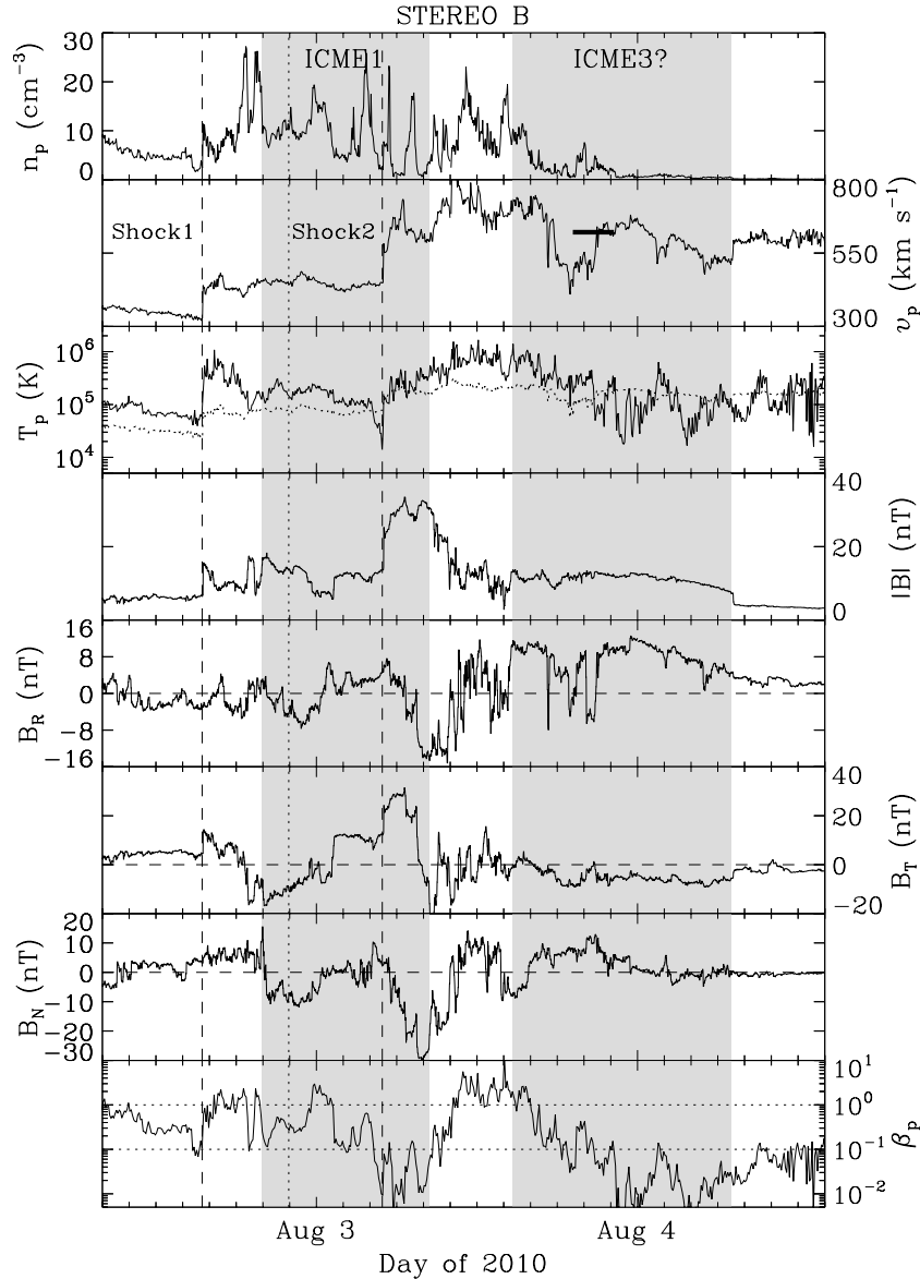
Figure 5. Similar to Figure 4, but for the measurements at STEREO B . ICME1 has a forward shock at STEREO B , while only a discontinuity is observed at Wind .
