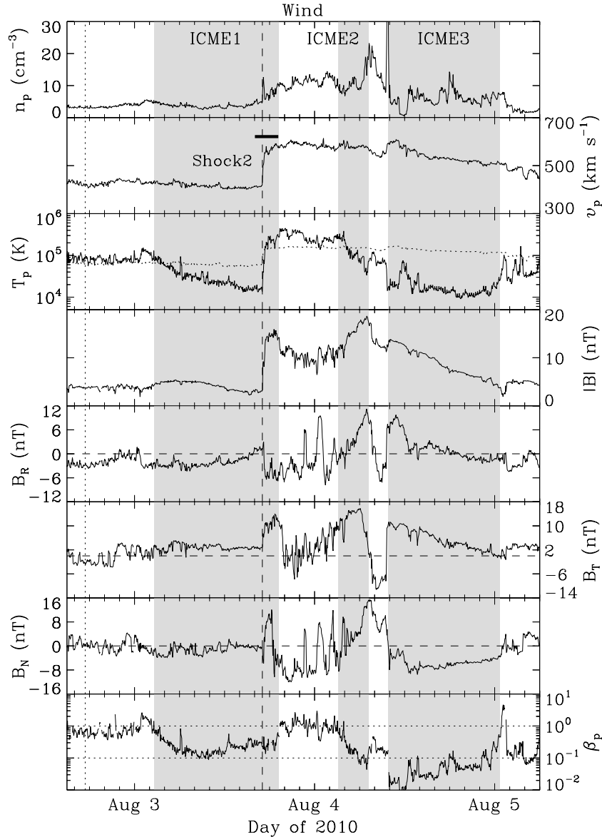
Figure 4. Solar wind plasma and magnetic field parameters observed at Wind . From top to bottom, the panels show the proton density, bulk speed, proton temperature, magnetic field strength and components, and proton \beta , respectively. The dotted curve in the third panel denotes the expected proton temperature from the observed speed. The shaded regions show the ICME intervals, and the vertical dashed line indicates the associated shock. The horizontal line in the second panel marks the predicted arrival time (with uncertainties) and speed of the merged front of CME2 and CME3 at the spacecraft. The predicted arrival time of CME1 is indicated by the vertical dotted line.
