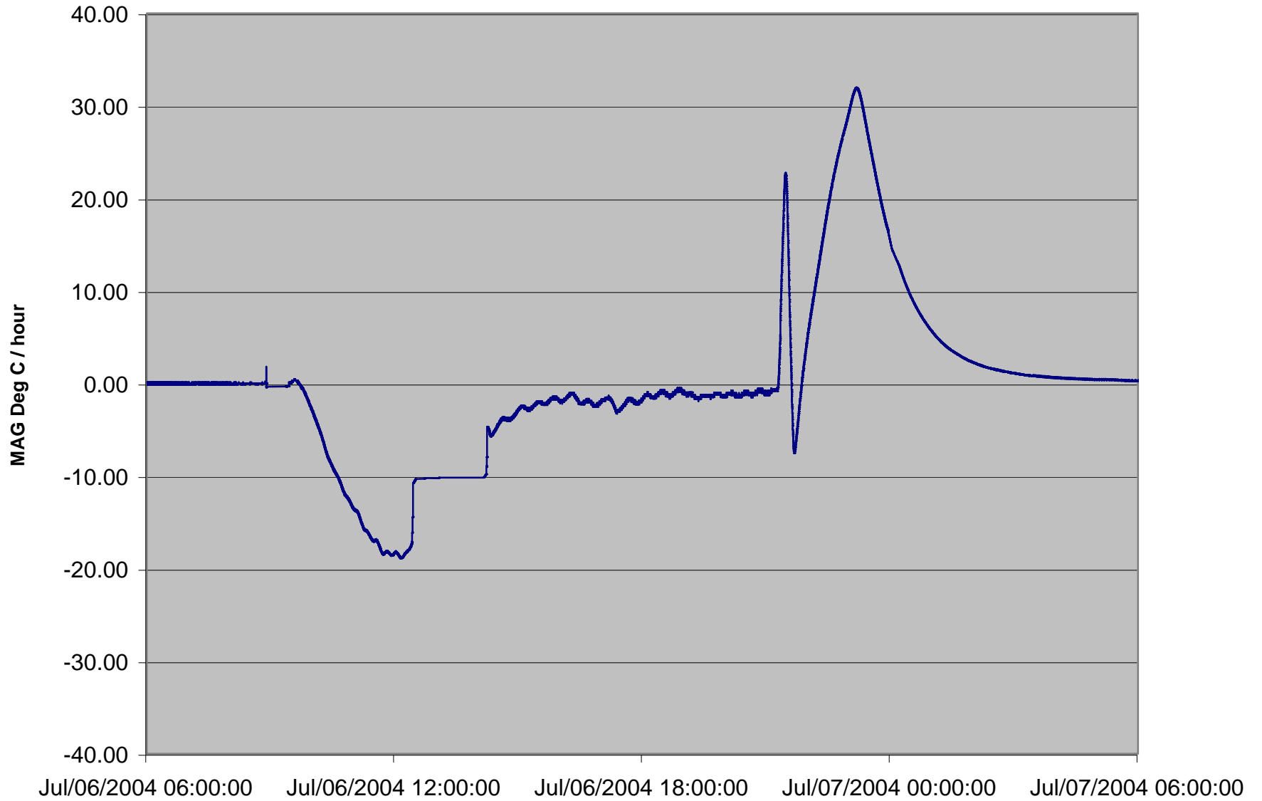
FM1 Boom Thermal Vac, Cycle 1
