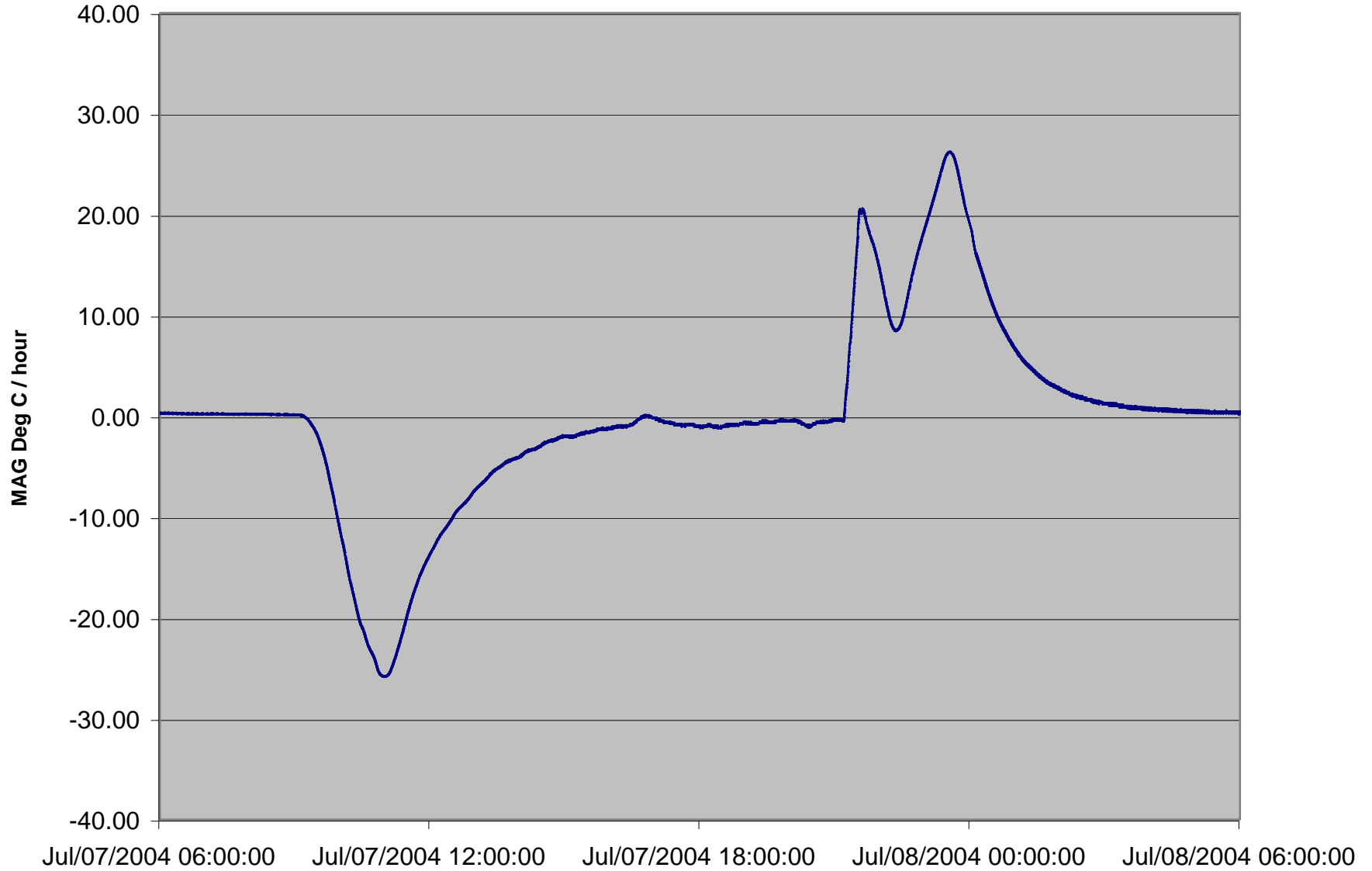
FM1 Boom Thermal Vac, Cycle 2
