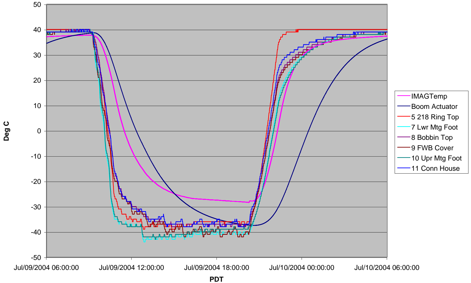
FM1 Boom Thermal Vac, Cycle #4
