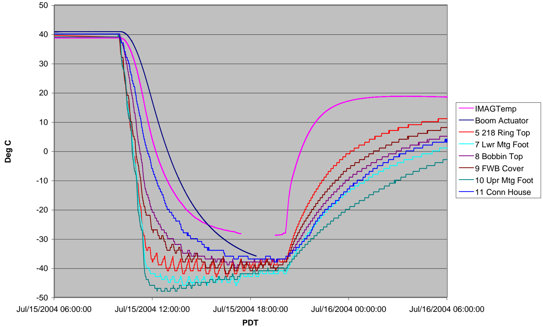
FM1 Boom Thermal Vac, Cycle #7, Cold Boom Deploy
