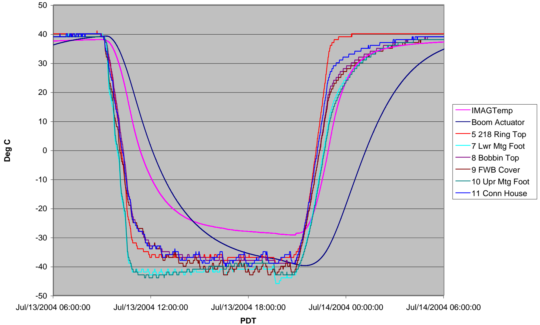
FM1 Boom Thermal Vac, Cycle #6
