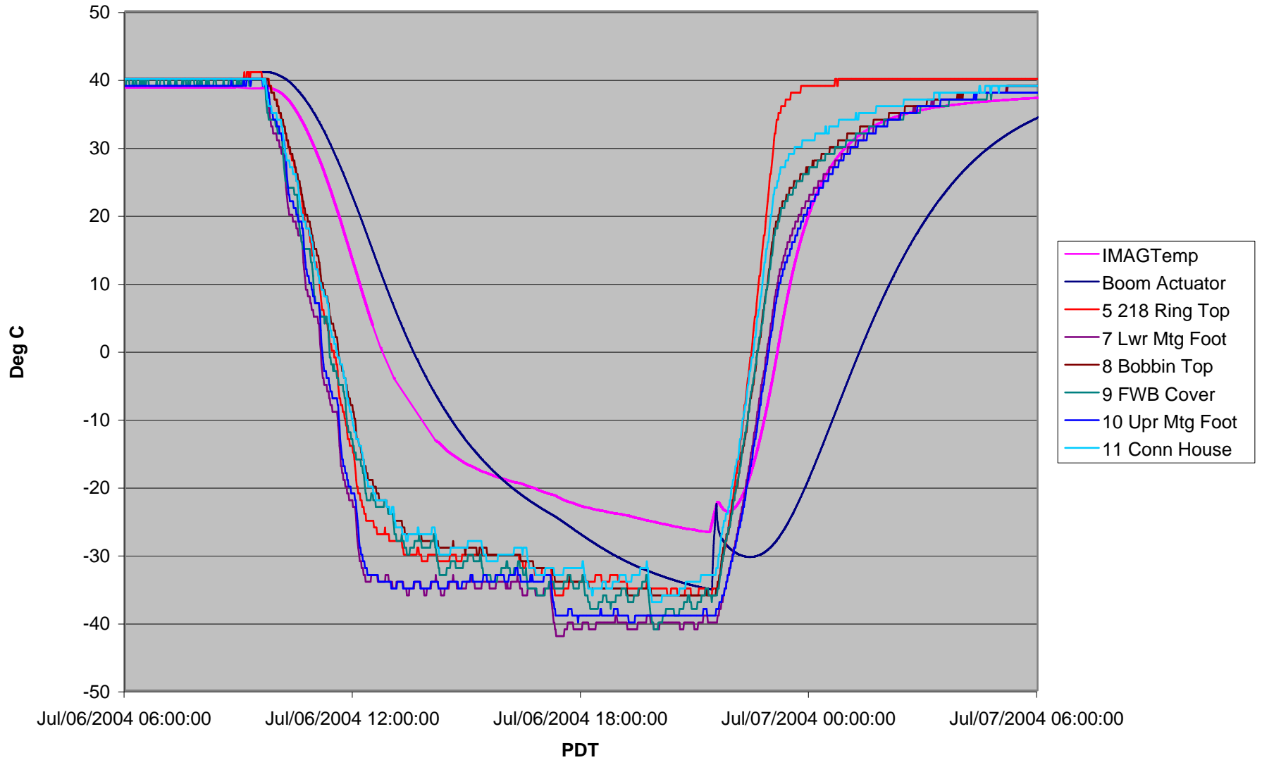
FM1 Boom Thermal Vac, Cycle #1
