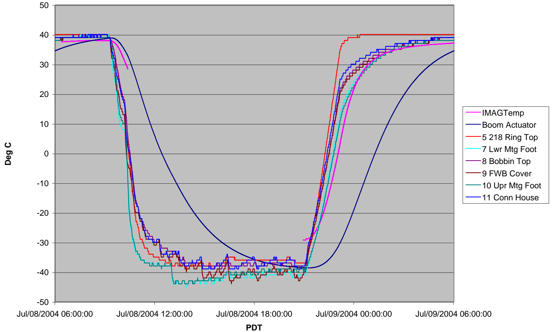
FM1 Boom Thermal Vac, Cycle #3
