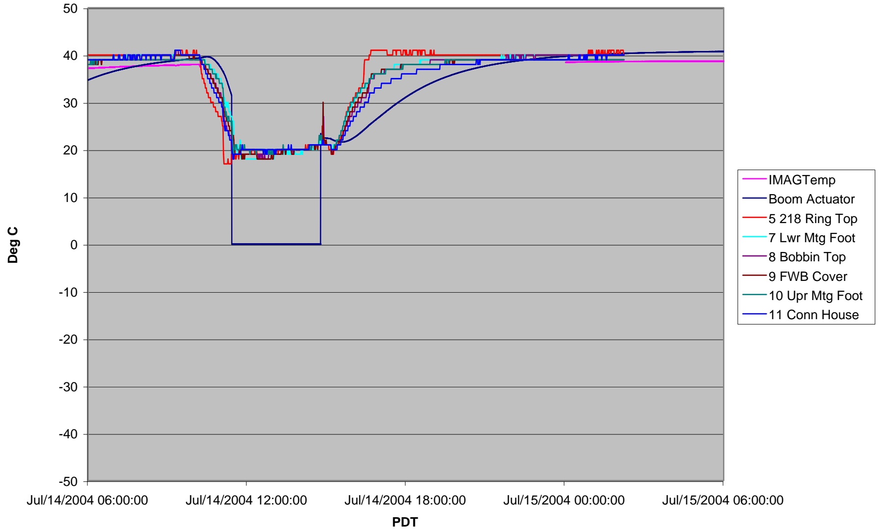
FM1 Boom Thermal Vac, Cycle #7, Hot Boom Deploy, Restow
