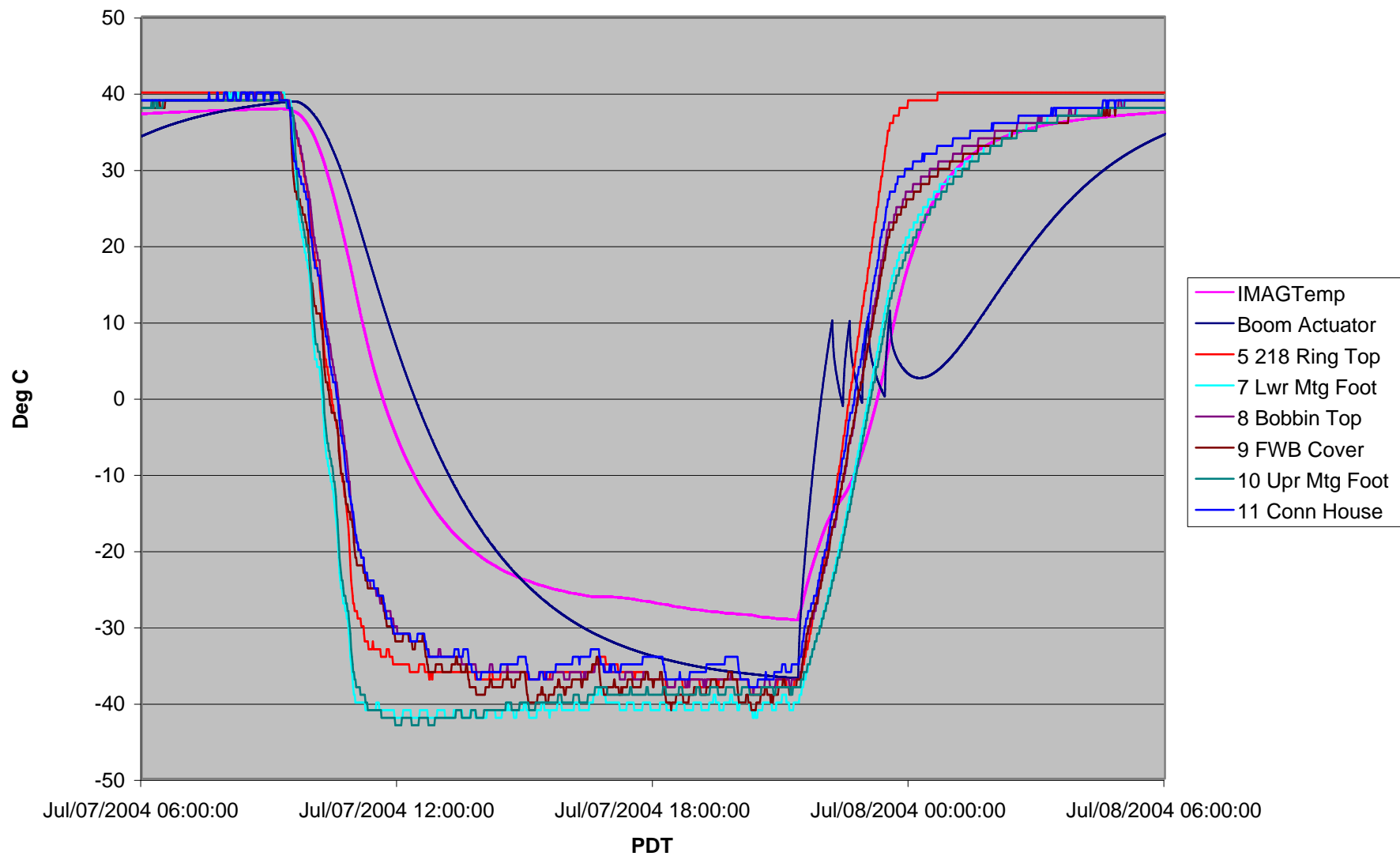
FM1 Boom Thermal Vac, Cycle #2
