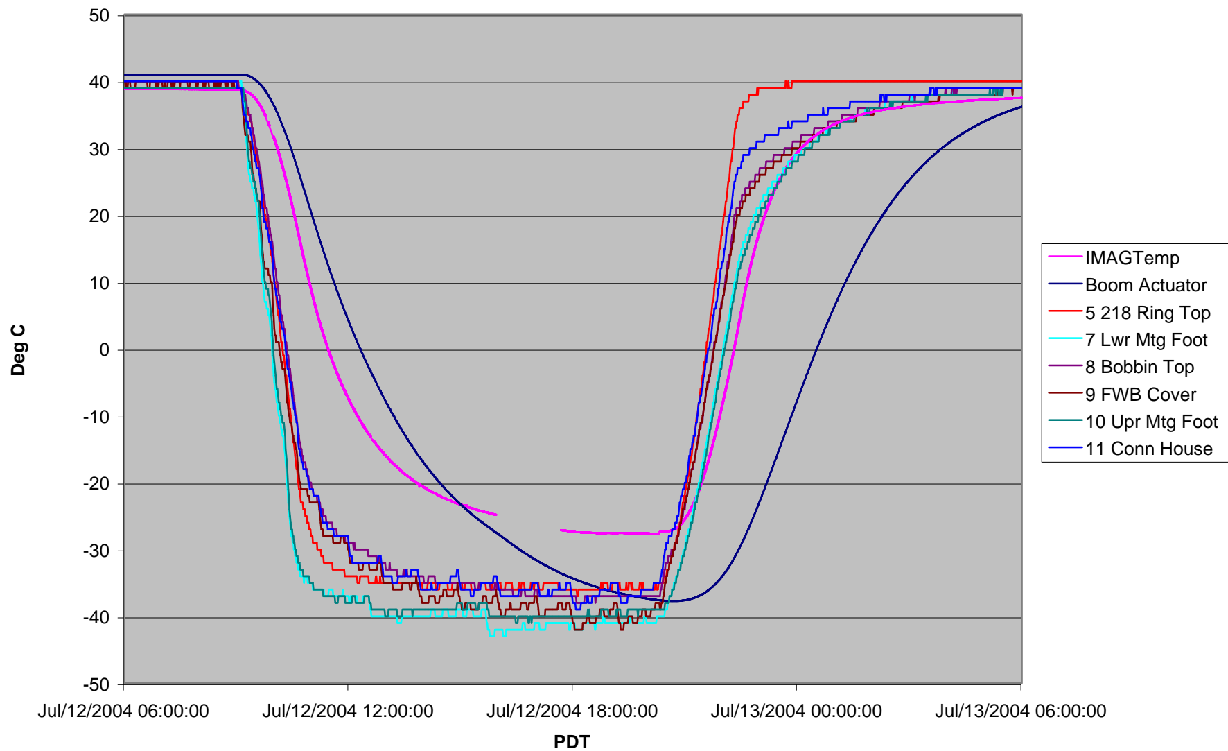
FM1 Boom Thermal Vac, Cycle #5
