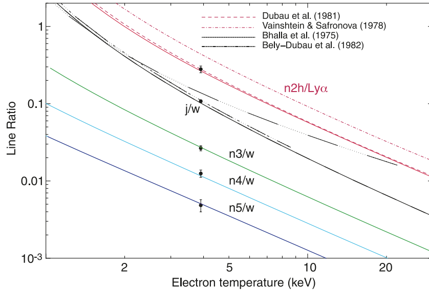
Fig. 4. Intensity ratios of DR satellite lines to resonance lines w and Ly_\alpha as functions of temperature. The solid circles with error bars are the measured data. The solid lines are the present calculations. The dashed and dash-dotted lines are the calculations of Dubau et al. [10] and of Vainshtein and Safronova [11] for the H-like satellite lines to Ly_\alpha ratio. The dotted and dash-dot-dot-dotted lines are the calculation of Bhalla et al. [6] and of Bely-Dubau et al. [9] for the He-like satellite line j to the resonance line w ratio.
