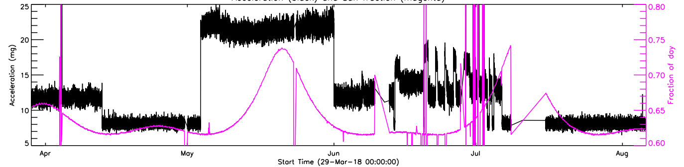
Acceleration (black) and Sun fraction (magenta)
