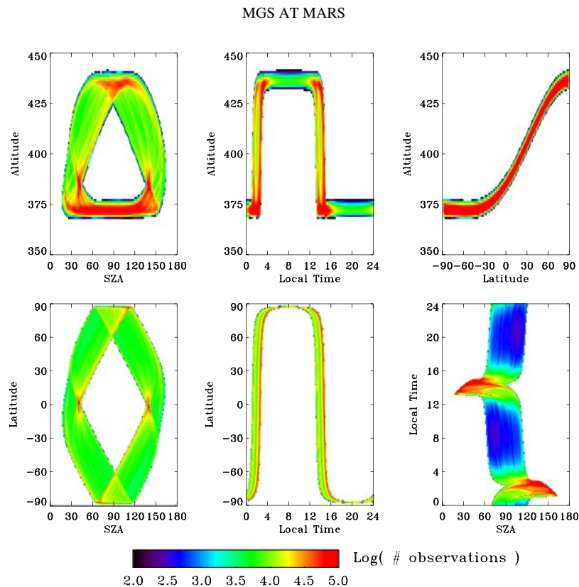
Figure 3. Data coverage for MGS MAG during mapping orbits from 2 June 1999 and 31 March 2004, in the same format as Figure 2.
