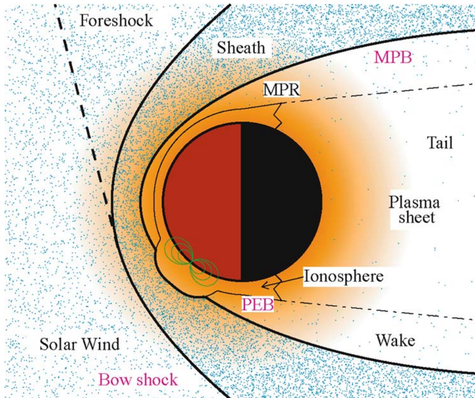
Figure 1. Cartoon of the global Martian solar wind interaction. Orange shading indicates density of planetary neutrals. Blue indicates relative density of solar wind ions in different plasma regions (labeled in black), separated by different plasma boundaries (labeled in magenta). Boundary names in this figure are those specific to MGS literature.
