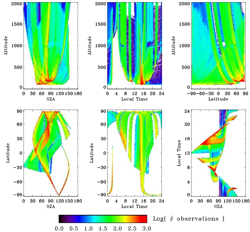
Figure 2. Data coverage for MGS MAG full vector measurements recorded during premapping orbits from 13 September 1997 through 28 January 1999. Panels show data density for times when the spacecraft was below 2000 km altitudes, as a function of altitude, solar zenith angle, local time, and latitude.
