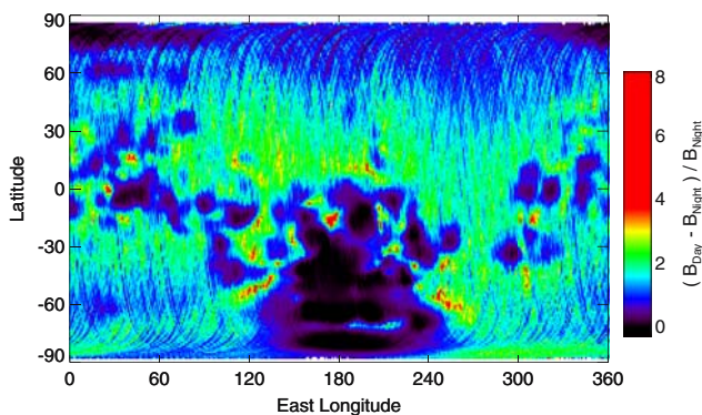
Figure 14. Geographic map of compression in the magnetic field magnitude, expressed as \Delta B/B_{\text{night}} , where \Delta B = B_{\text{day}} - B_{\text{night}} .
