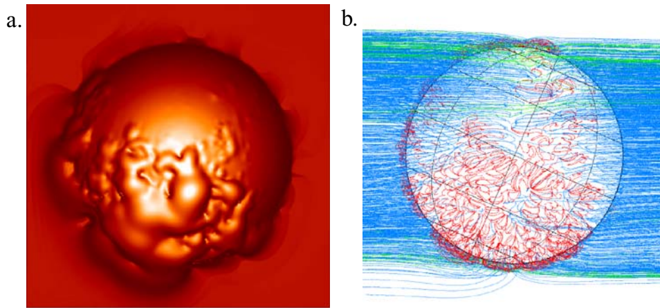
Figure 5. Cartoon showing: (a) the Martian pressure balance obstacle and (b) magnetic field topology. (a) The shape of the Martian solar wind obstacle is derived from a calculation of pressure balance between upstream solar wind dynamic pressure and a combination of ionospheric thermal pressure and magnetic pressure from crustal fields. (b) The magnetic field topology results from field line tracing in a vacuum superposition of a crustal field model with a uniform background magnetic field. Field lines are colored according to their topology: closed (red), open (blue), or draped (green). Mars has the same orientation in both panels. From Brain (2002).
