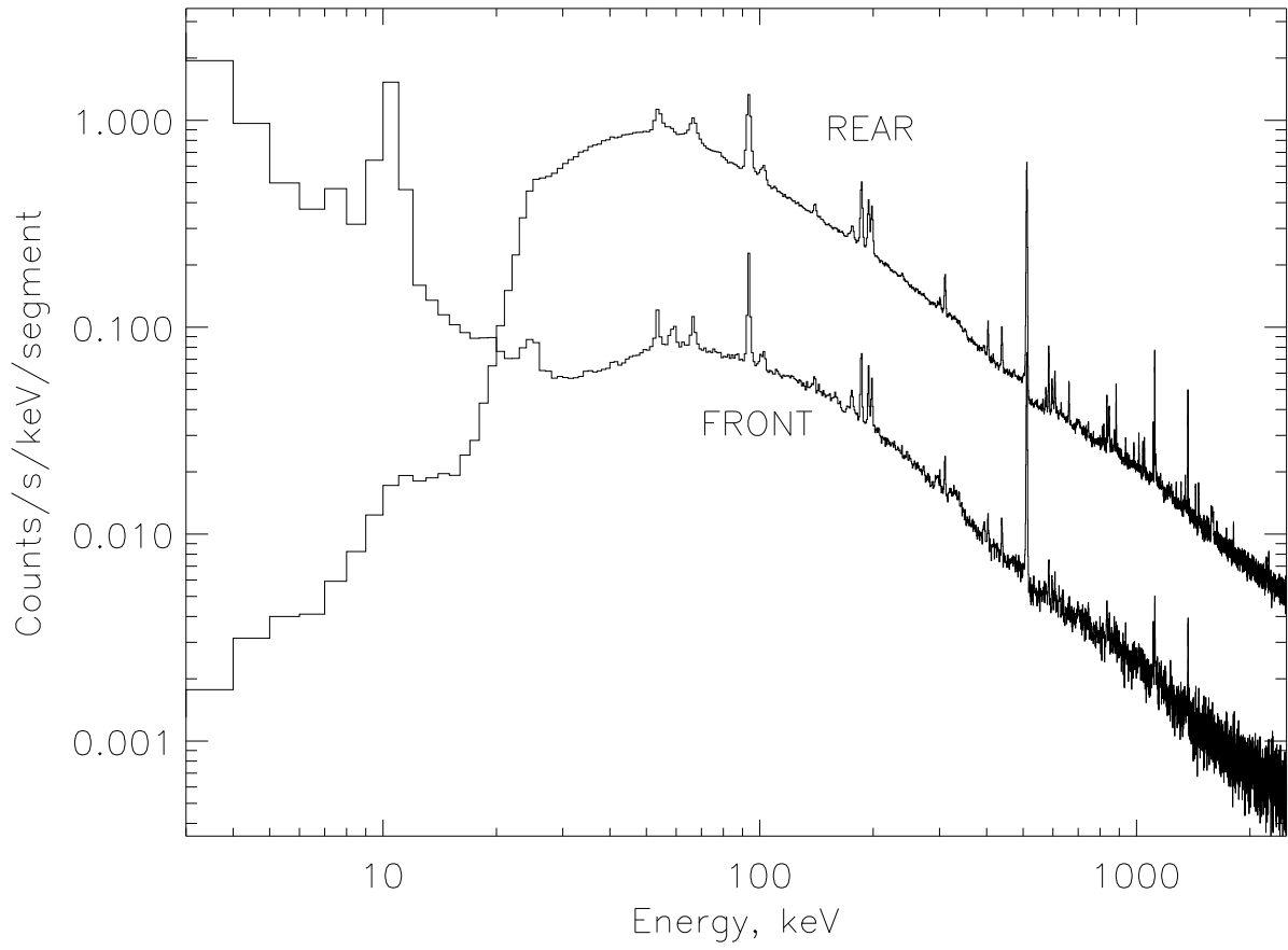
RHESSI average background
