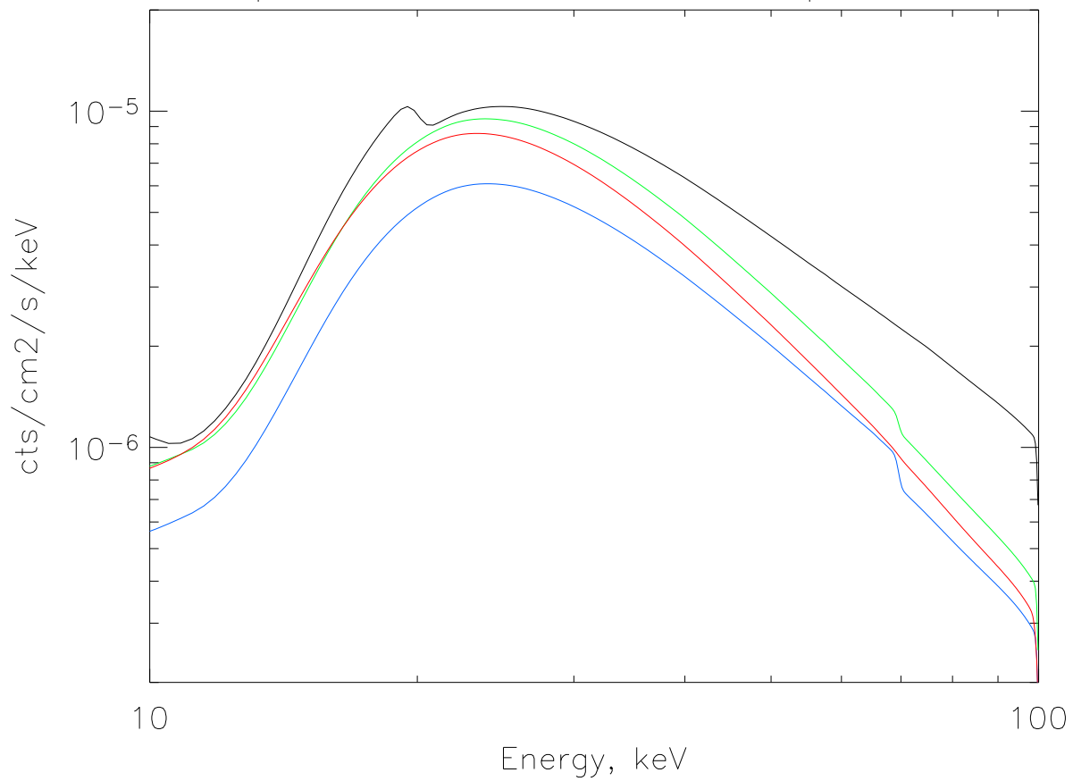
Response of G1,3,4,5 to E^{-3} power law
