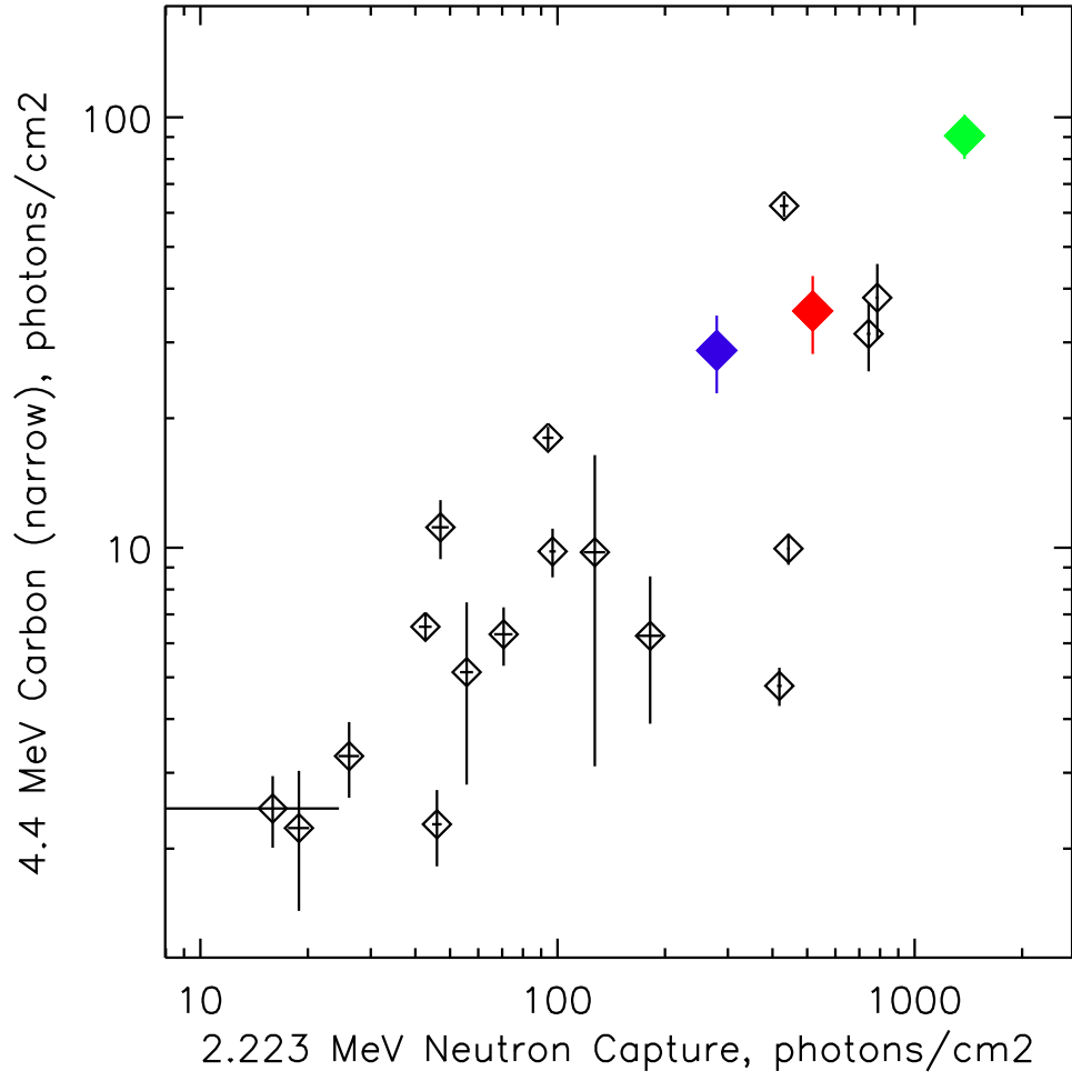
SMM & RHESSI Fluences, Corrected
