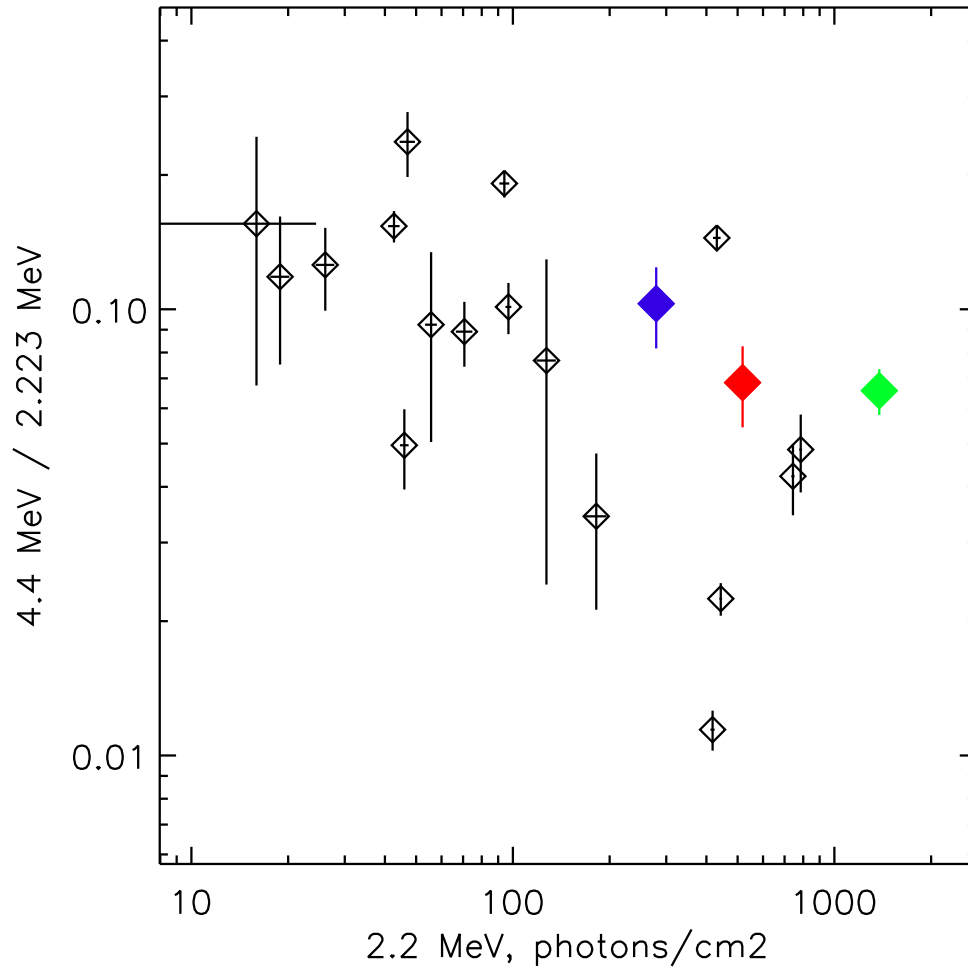
SMM & RHESSI Ratios, Corrected
