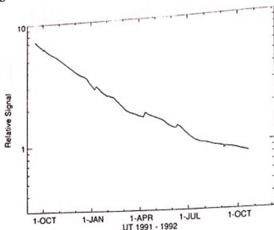
FIGURE 2. Relative signal level for Yohkoh white-light images, showing the steady decrease of signal level during the duration of the observations. The necessary exposure time grew from about 60 msec to about 948 msec during this period. The sudden increases occurred when the CCD was warmed up to drive off contaminants from its surface.
