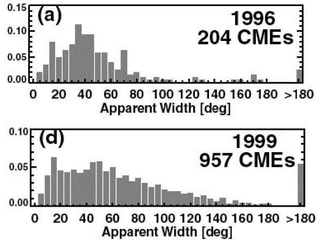
Figure 4. Angular sizes of CMEs vs. phase in the solar cycle, based upon LASCO observations (St. Cyr et al., 2000). The numbers of wider CMEs increases towards the solar maximum (Hundhausen, 1993).
