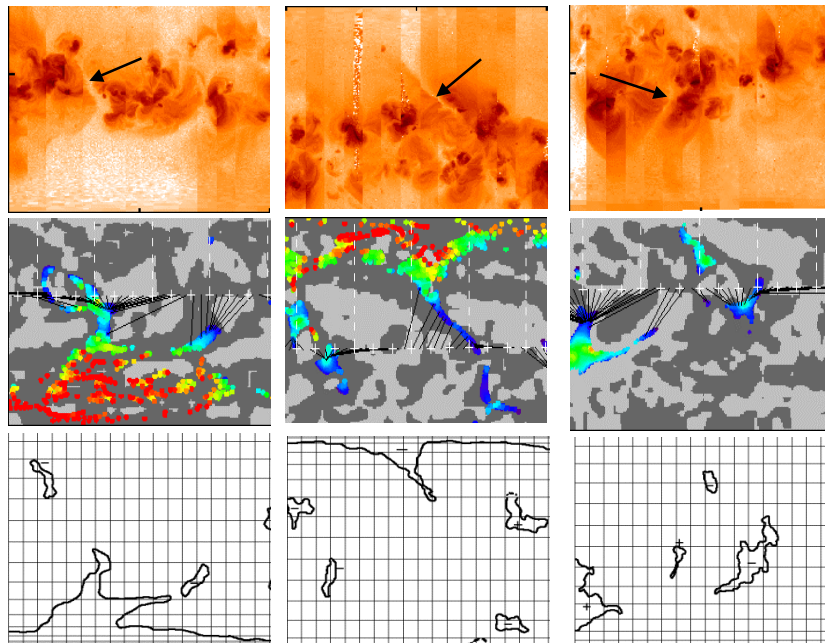
FIGURE 2. Synoptic maps (top, Yohkoh soft X-rays; middle, model magnetic field; and bottom, HE I 10830Å CH boundary map) for each of the three NCH episodes studied (left, CR 1851, the “YCHI” of [9]; middle, CR 1982; right, CR 1983). The arrows in the X-ray images point to the NCHs discussed in this paper. The colored dots represent photospheric footpoints of open field lines, with different colors used to indicate the expansion factors (or solar wind speed) associated with the flux tubes. Red corresponds to small expansion factors or fast wind, while blue corresponds to large expansion factors or slow wind. Areas shaded light gray (dark gray) are closed field lines with B_r > 0 ( B_r < 0 ).
