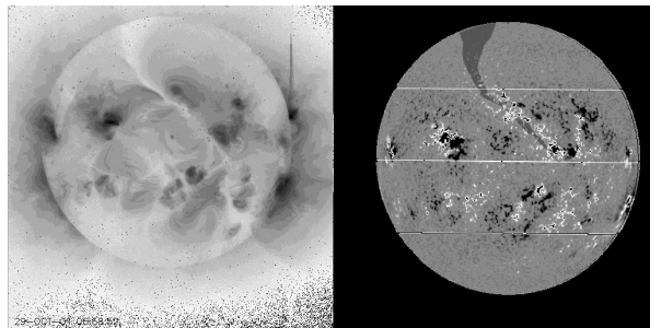
FIGURE 1. Representative narrow coronal hole (NCH) observed by Yohkoh , 29 October 2001. The north polar hole can be seen to extend to the southwest (lower right) into a strong-field region towards NOAA region 9678 (N07, W21), as shown in the rough overlay over the KPNO magnetogram on the right.
