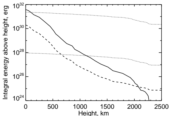
Fig. 19 The energy contained in the chromosphere, according to the VAL-C model (Vernazza et al. 1981), evaluated for an area 10^{18} cm 2 : dashed line, thermal energy; solid line, latent heat of ionization; dotted lines, total magnetic energy for uniform fluxes of 30 and 1500 G.
