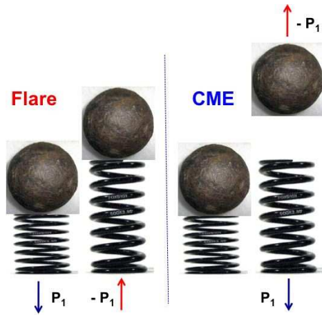
Fig. 15 Conservation of momentum, comparing an idealized flare and CME, inspired by Klimchuk (2001). For a CME the mass and momentum never return, but for a flare the evaporative motion is arrested by the closed field. Note that in this view the flare creates twice as much momentum as a CME of equal mass and ejection velocity, but in two episodes with equal and opposite signs. Note that illustrating momentum with a cannonball misrepresents the important component present in the wave field.
