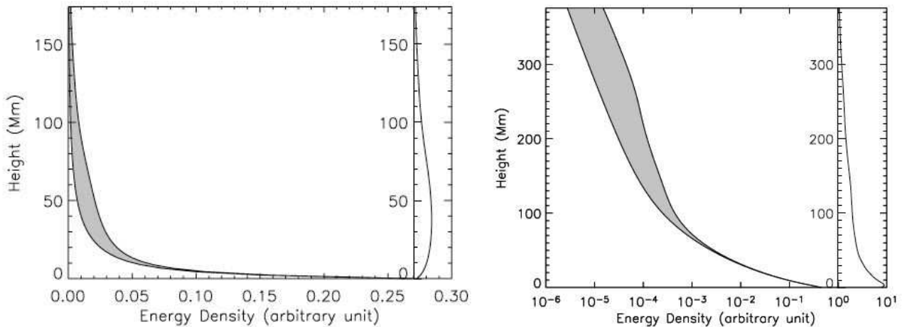
Fig. 21 The results of potential (lower curves) and non-linear force-free (upper curves) extrapolations from photospheric vector field measurements from Régnier and Priest (2007) for two solar active regions (NOAA AR 8151 and 8210, respectively). The inset plots show the variation of non-potential energy density with height
