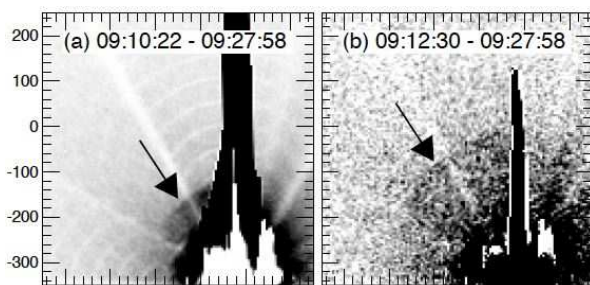
Fig. 11 A global coronal wave seen in soft X-rays with the Yohkoh/SXT telescope (adapted from Khan and Aurass 2002). Many image artifacts appear here because of the long exposure needed to capture the faint X-ray wave signatures marked with arrows; disregard the spokes, the light concentric rings, and the vertical spikes. The flare is at lower right in the image; the left major tick mark on the X-axis is at -100'' .
