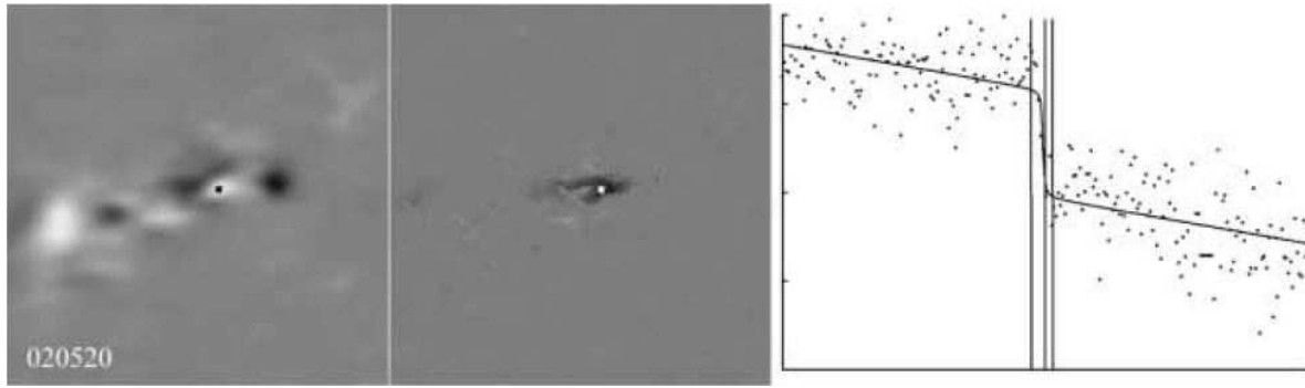
Fig. 22 One of the examples of stepwise changes in the photospheric longitudinal magnetic field by Sudol and Harvey (2005) as “ubiquitous features of X-class flares.” Left : a GONG longitudinal magnetogram (10-m average prior to the event) for the flare SOL2002-05-20T15:29 (X2.1, S21 E65); middle : a representation of the field change across the flare time; right : the field variation in a representative pixel. In the time-series plot the vertical lines denote the GOES start, peak (15:29 UT), and end times. The total duration of the plot is four hours, and the vertical scale spans 400 G.
