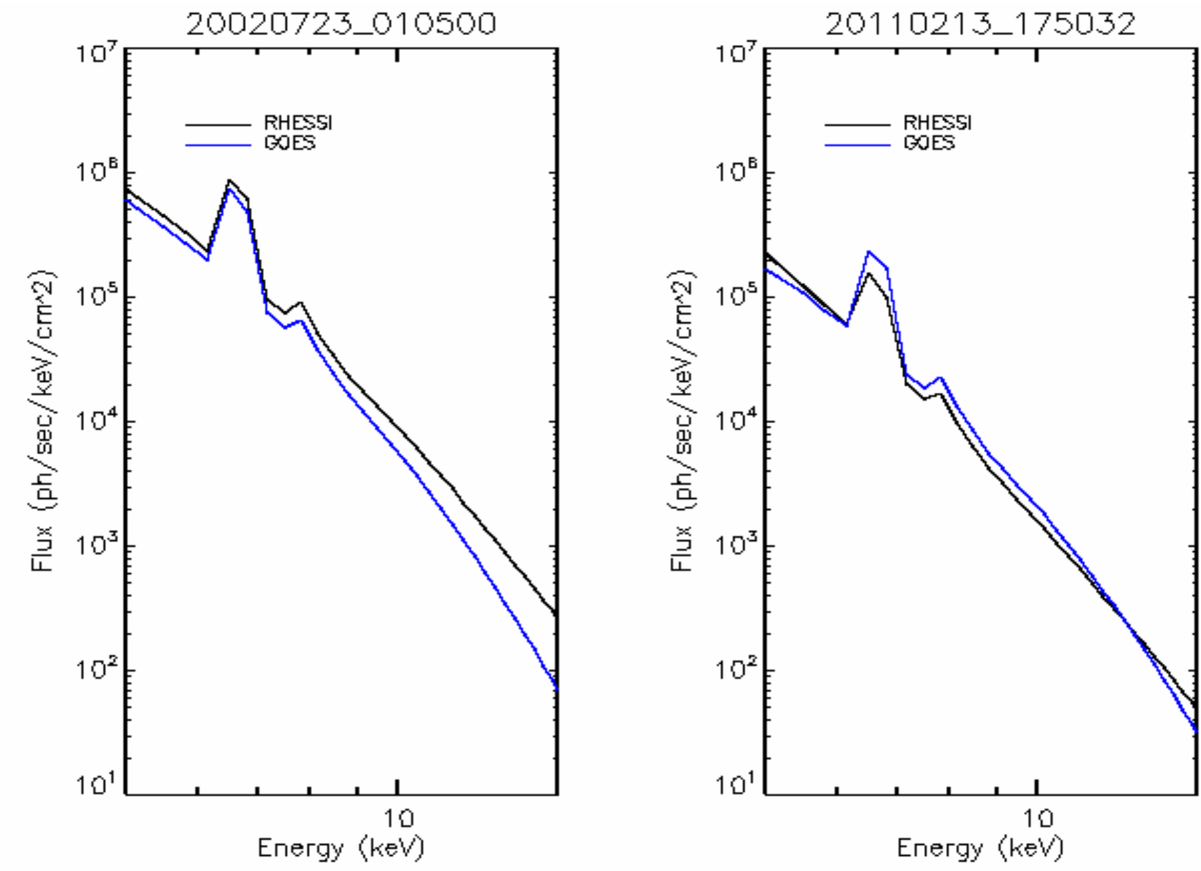
Figure 1: Comparison of photon flux for RHESSI spectral fits (black) with photon flux inferred from GOES-derived T and EM values (blue) for 2002 July 23, 01:05:00 UT to 01:06:00 UT (left) and 2011 February 13, 17:50:32 UT to 17:51:32 UT (right).
