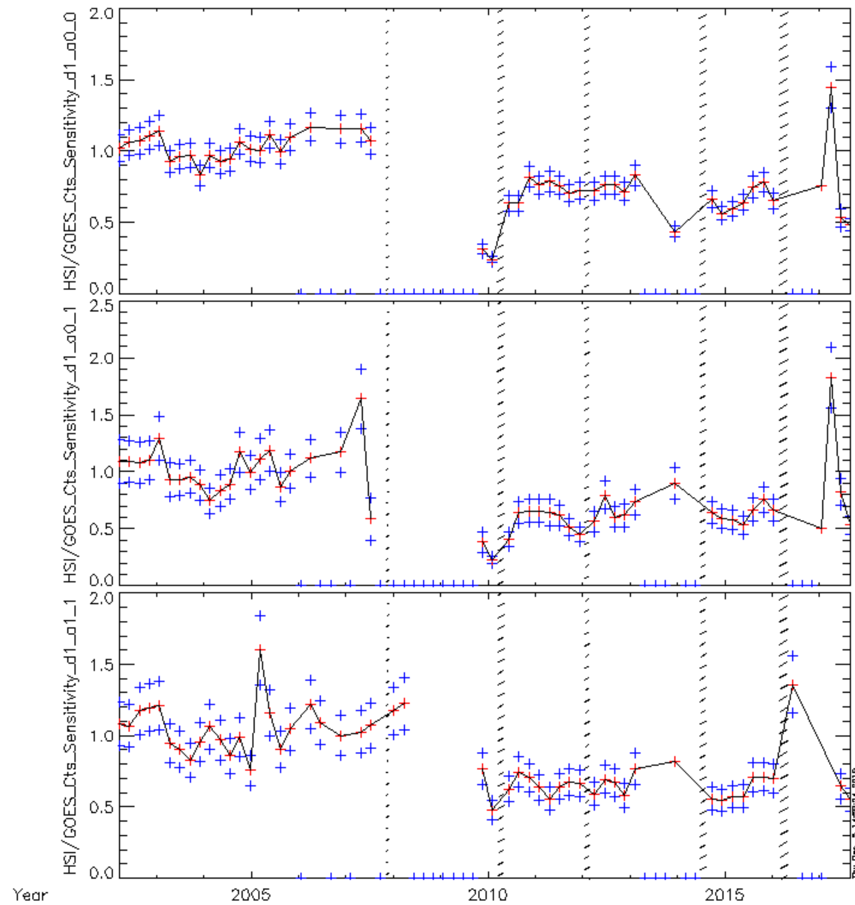
Figure 2: Normalized RHESSI/GOES sensitivity for RHESSI detector 1. The top and middle panels are for the energy bands 3 to 6 and 6 to 9 keV, with attenuator state 0. The bottom panel is for the 6 to 9 keV energy band, in attenuator state 1. Blue plusses show the standard deviation in each 80 day interval. The angled lines overlaid denote anneal periods. Detector 1 shows the least sensitivity loss.
