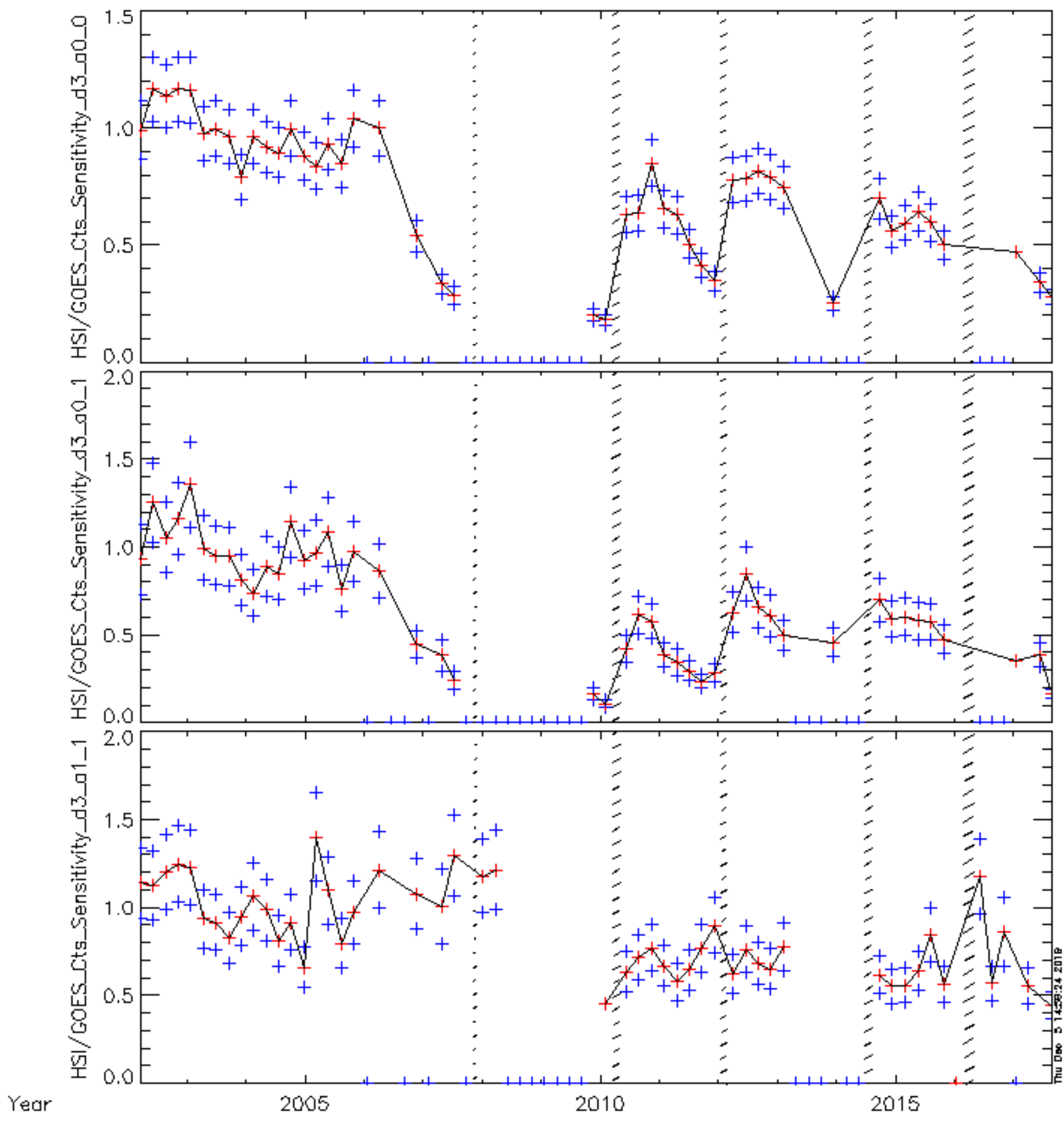
Figure 3: Normalized RHESSI/GOES sensitivity for RHESSI detector 3. The top and middle panels are for the energy bands 3 to 6 and 6 to 9 keV, with attenuator state 0. The bottom panel is for the 6 to 9 keV energy band, in attenuator state 1. Blue plusses show the standard deviation in each 80 day interval. The angled lines overlaid denote anneal periods. Detector 3 shows noticeable sensitivity loss, especially for attenuator state of 0.
